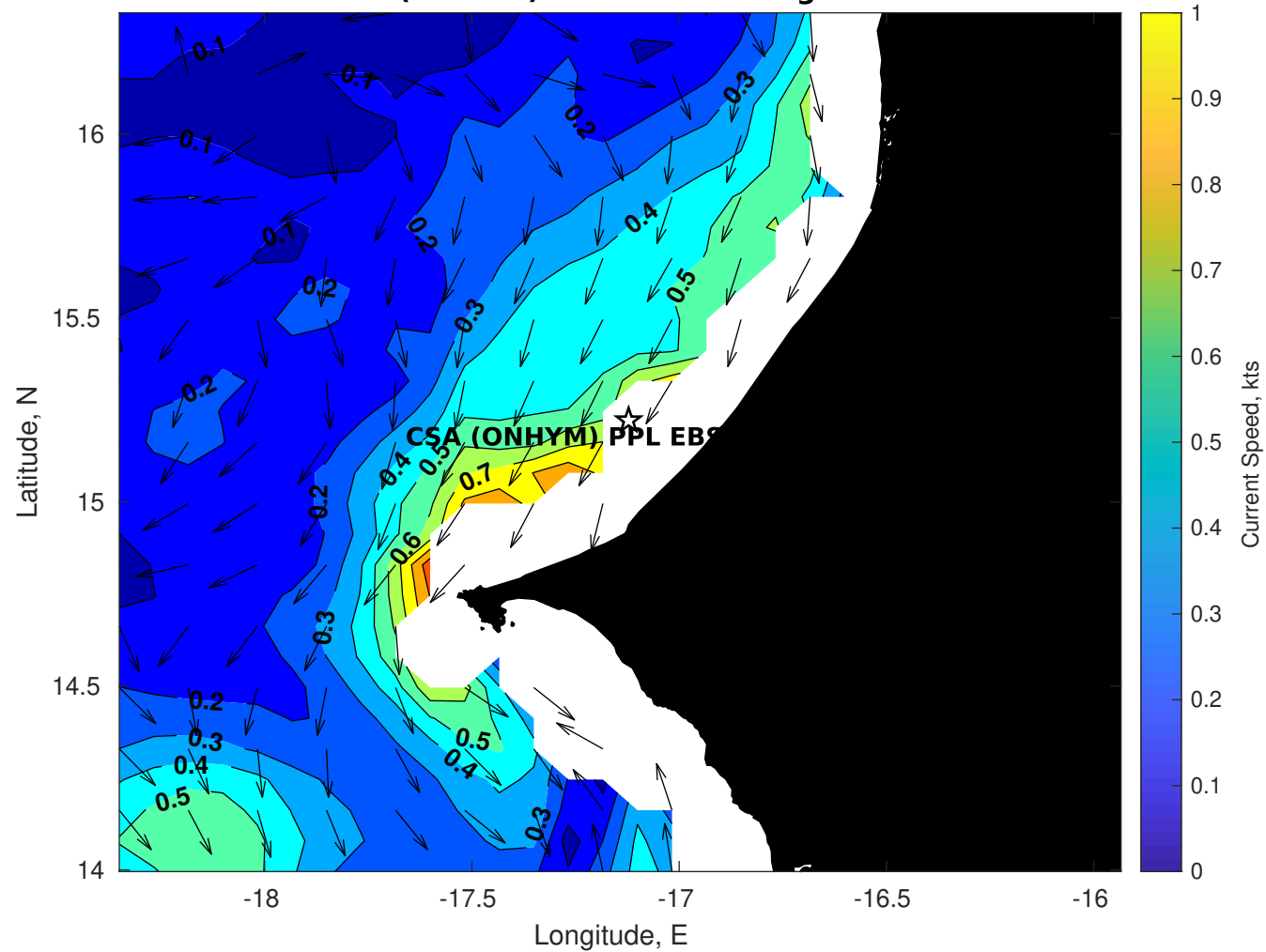
Surface Currents for CSA (ONHYM) PPL EBS - Senegal at 03-Nov-2025 00:00:00
