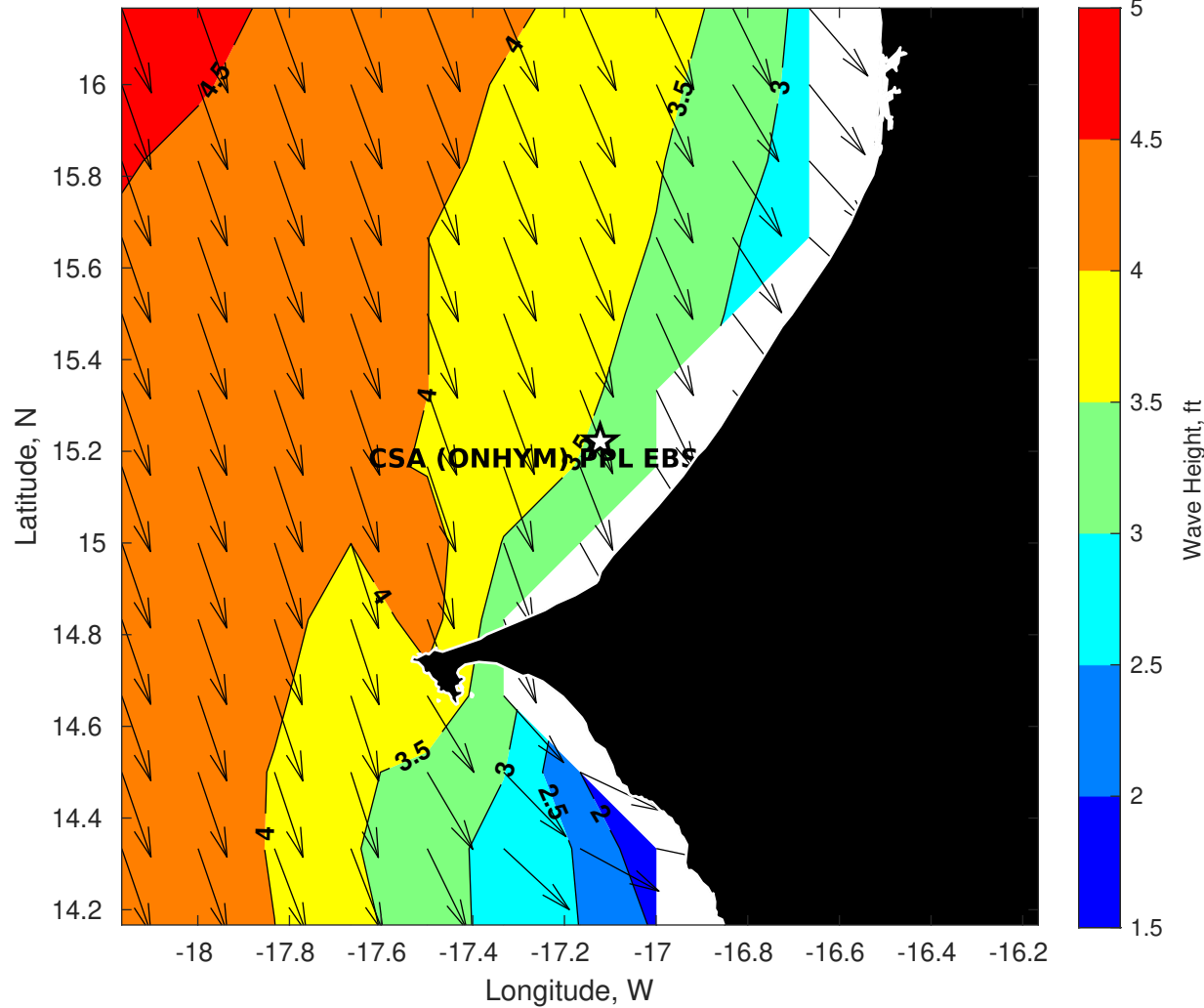
Wave Height (ft) for CSA (ONHYM) PPL EBS - Senegal at 04-Nov-2025 09:00:00
