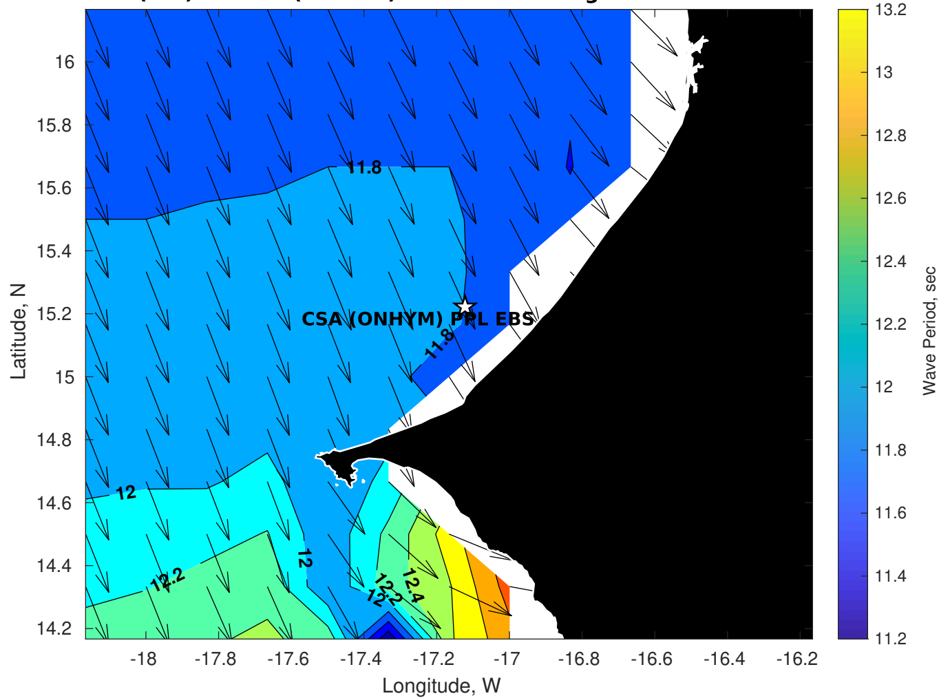
Wave Period (sec) for CSA (ONHYM) PPL EBS - Senegal at 04-Nov-2025 09:00:00
