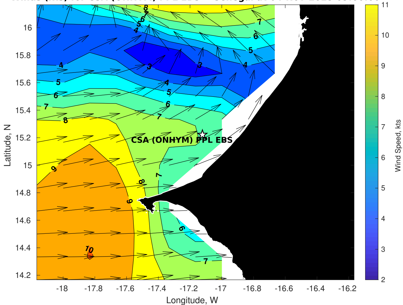
Winds (kts) for CSA (ONHYM) PPL EBS - Senegal at 04-Nov-2025 09:00:00
