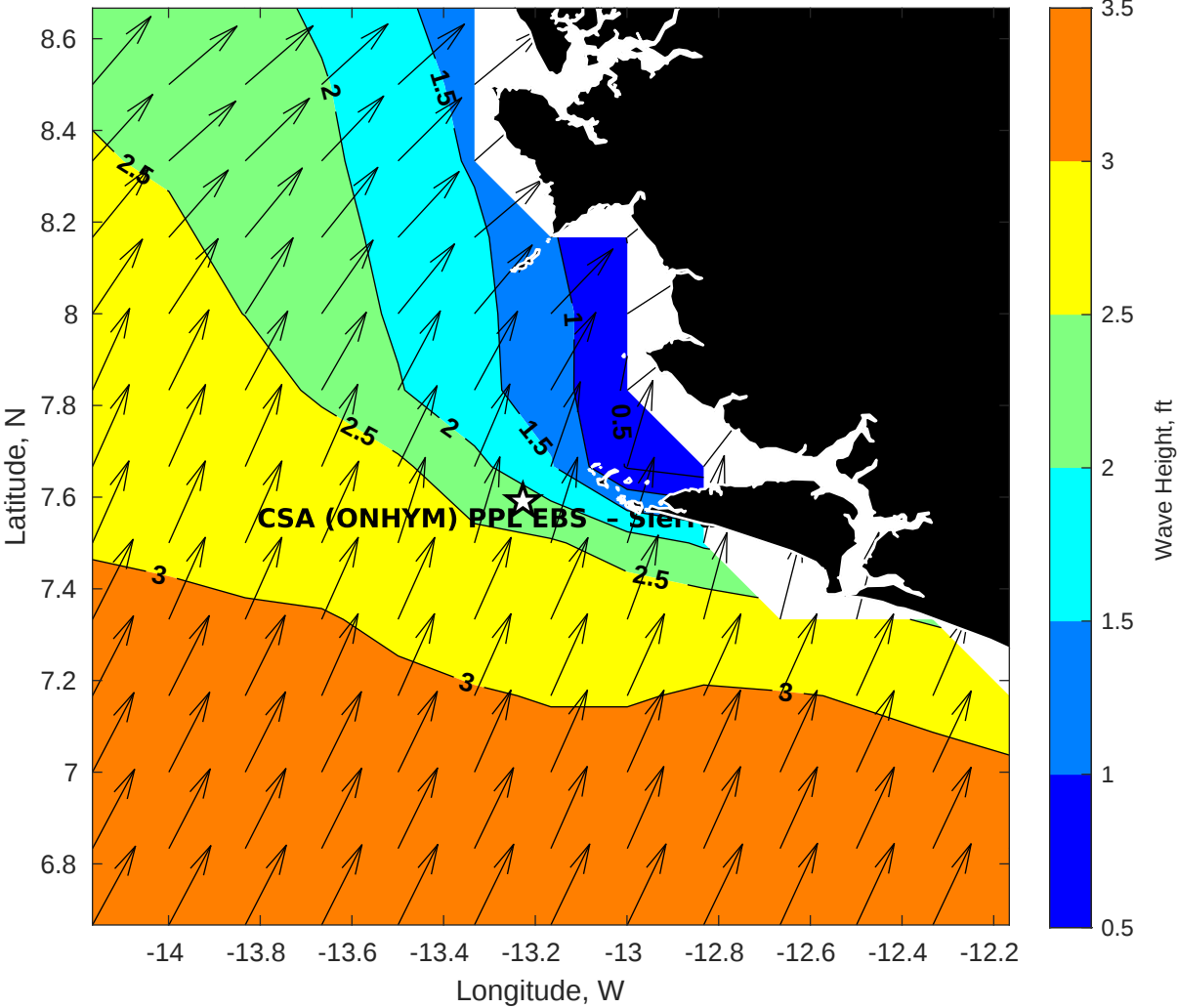
Wave Height (ft) for CSA (ONHYM) PPL EBS - Sierra Leone at 04-Nov-2025 09:00:00
