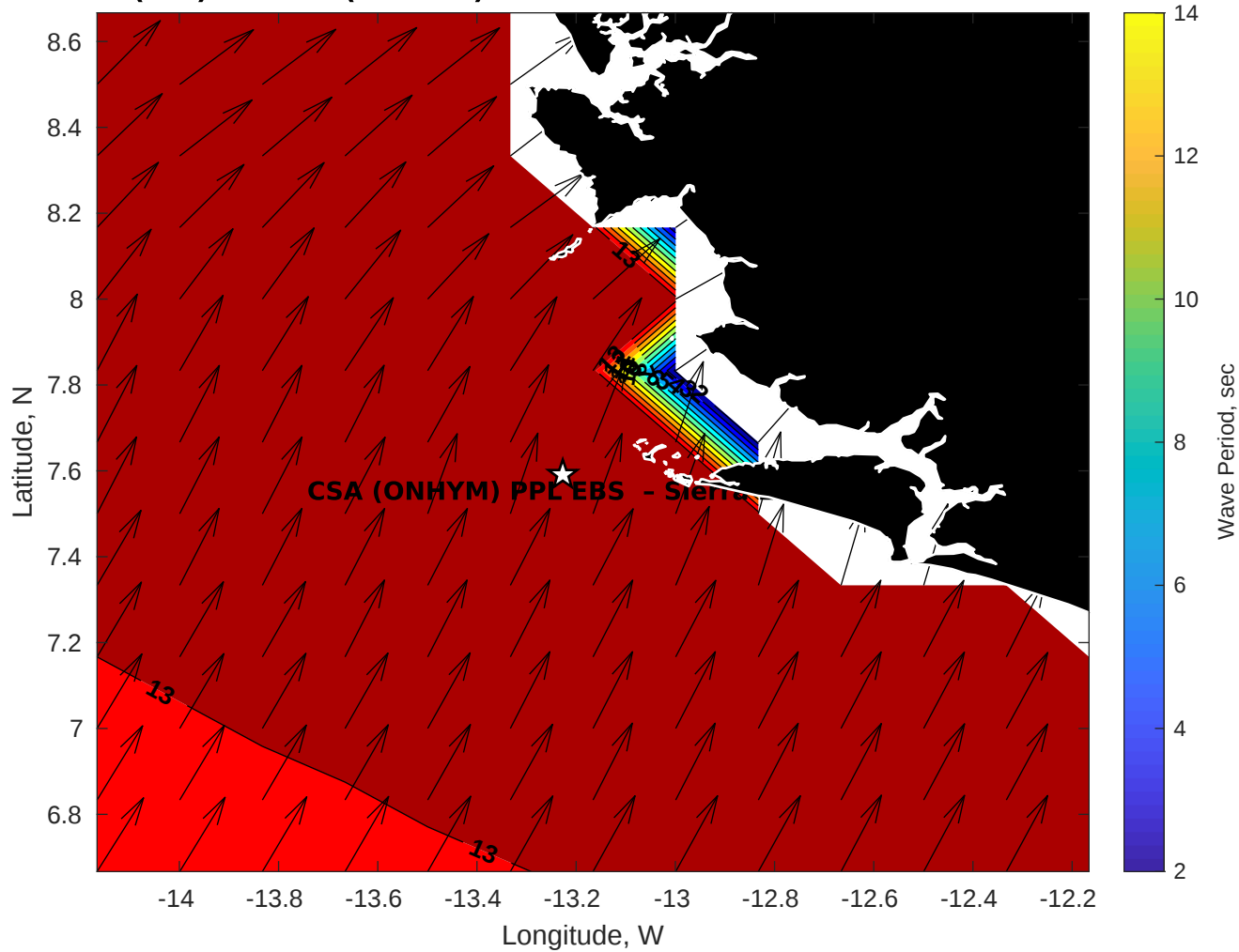
Wave Period (sec) for CSA (ONHYM) PPL EBS - Sierra Leone at 04-Nov-2025 09:00:00
