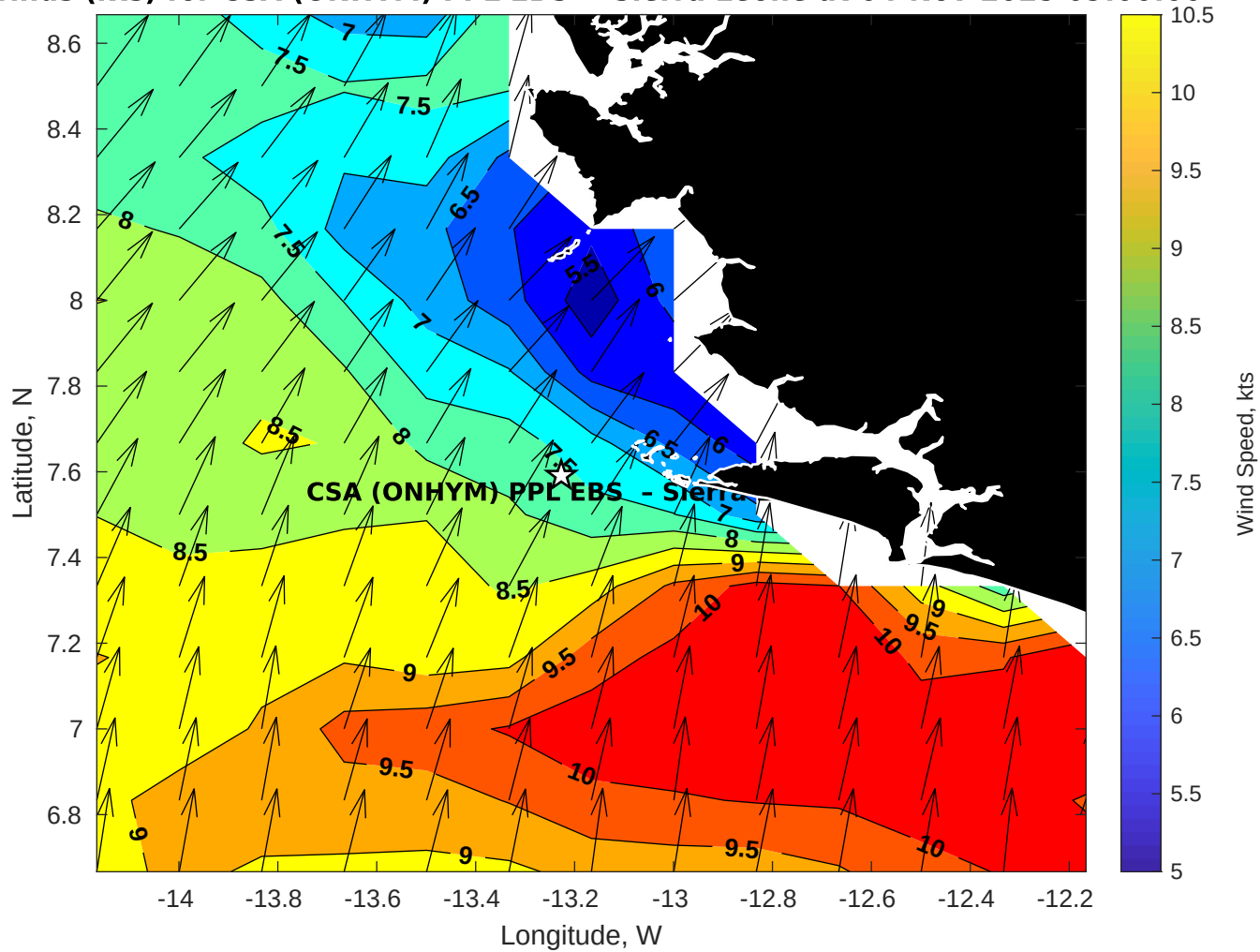
Winds (kts) for CSA (ONHYM) PPL EBS - Sierra Leone at 04-Nov-2025 09:00:00
