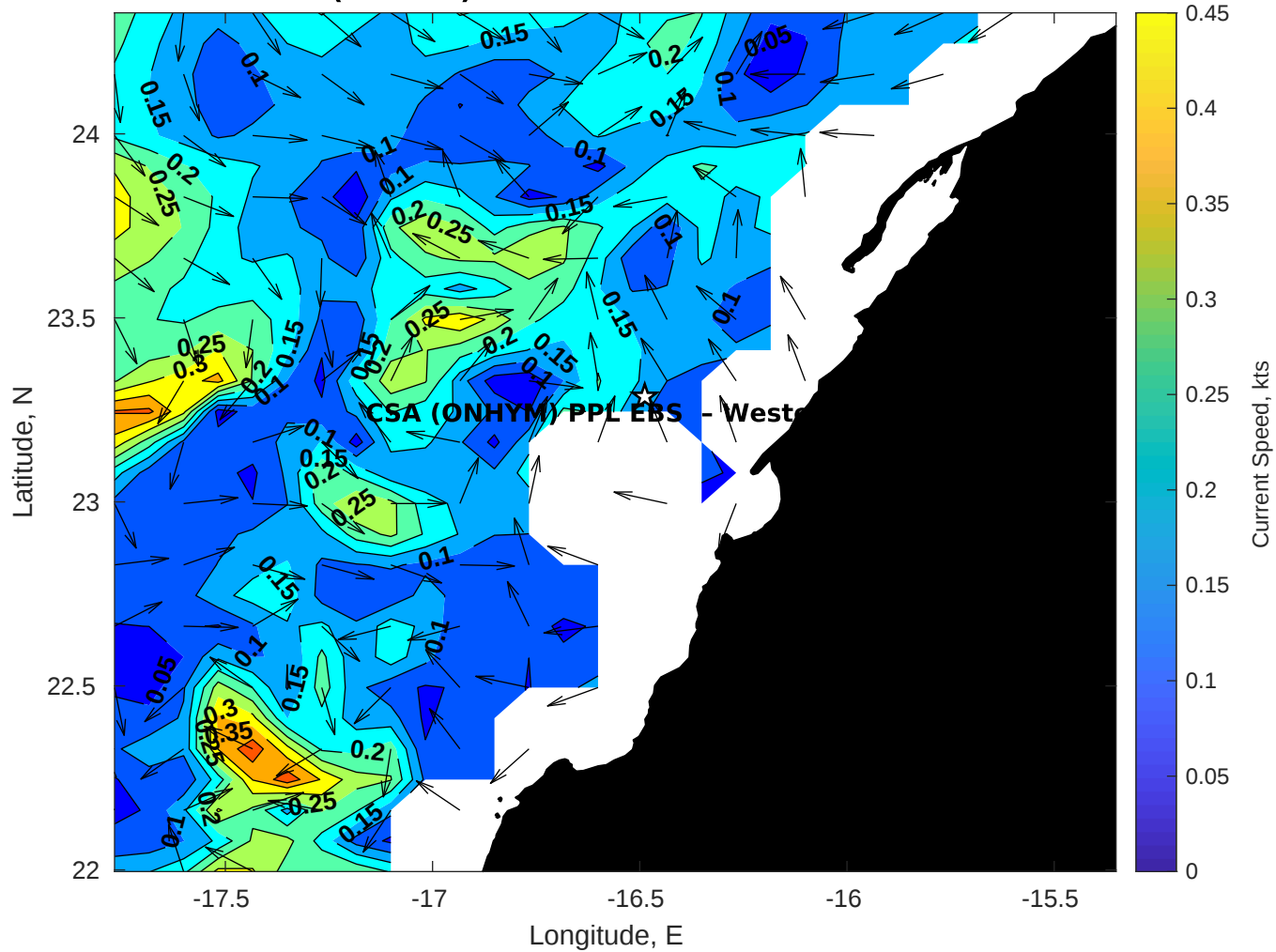
Surface Currents for CSA (ONHYM) PPL EBS - Western Sahara at 03-Nov-2025 00:00:00
