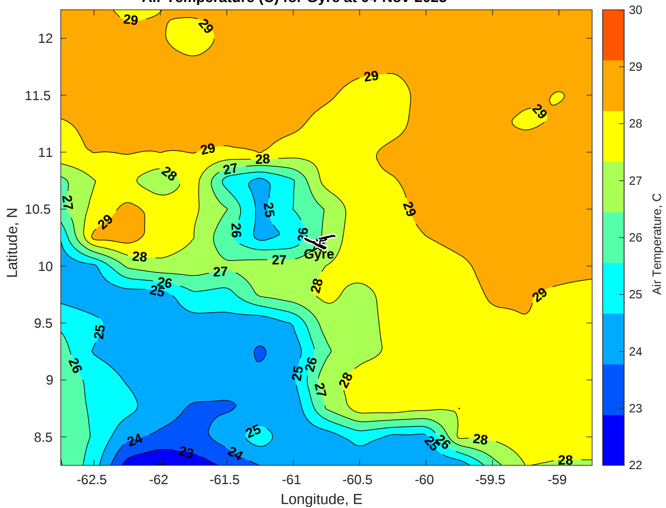
Air Temperature (C) for Gyre at 04-Nov-2025
