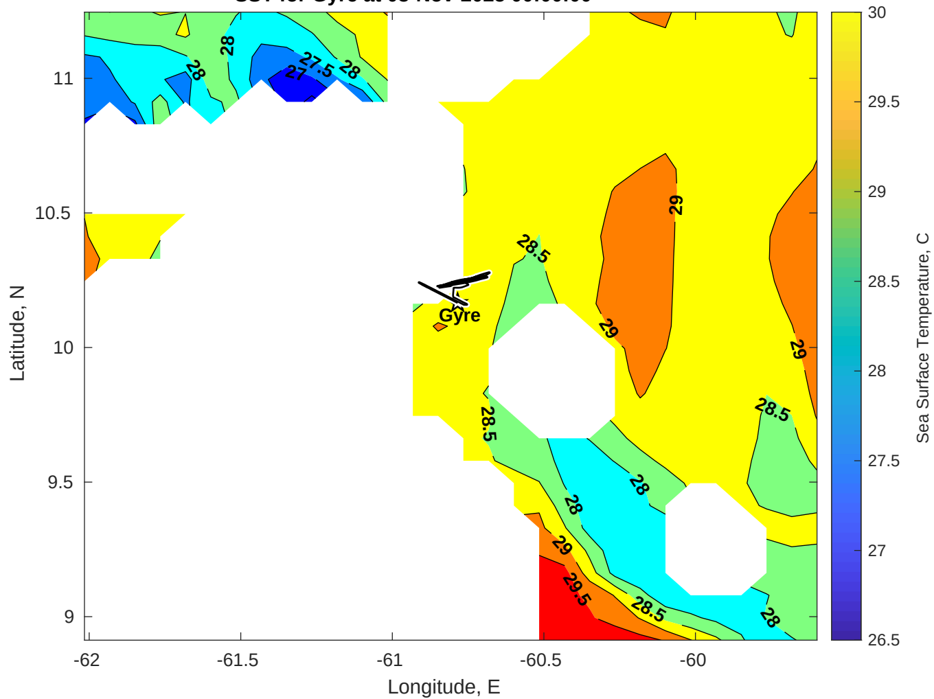
SST for Gyre at 03-Nov-2025 00:00:00
