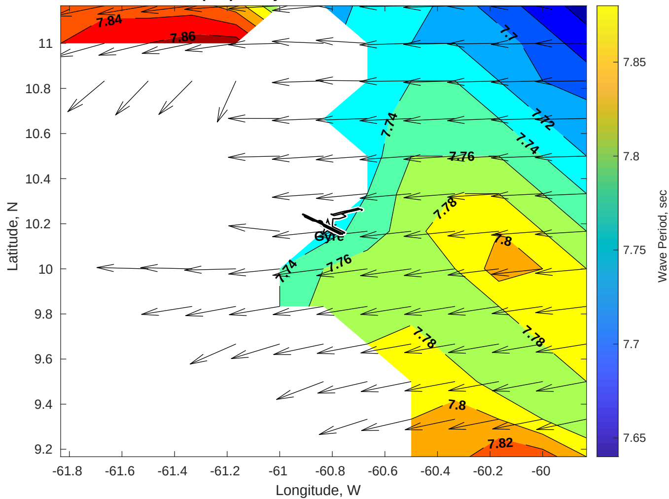
Wave Period (sec) for Gyre at 04-Nov-2025 09:00:00
