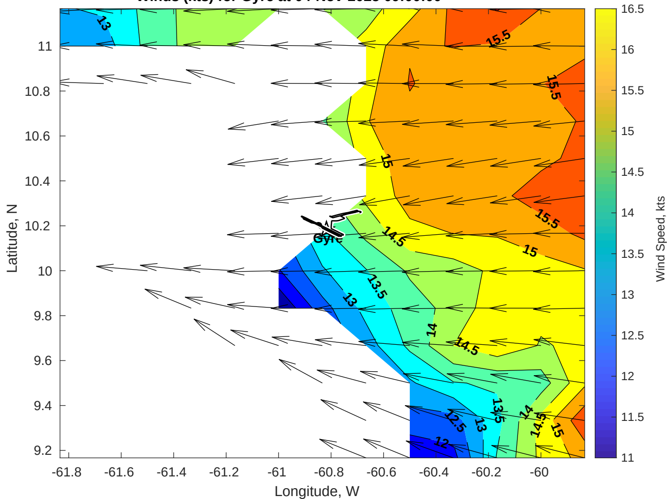
Winds (kts) for Gyre at 04-Nov-2025 09:00:00
