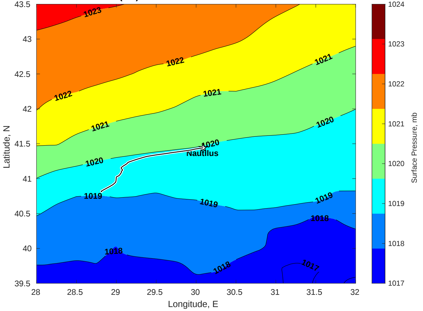
Surface Pressure (mb) for Nautilus at 06-Nov-2025 00:00:00
