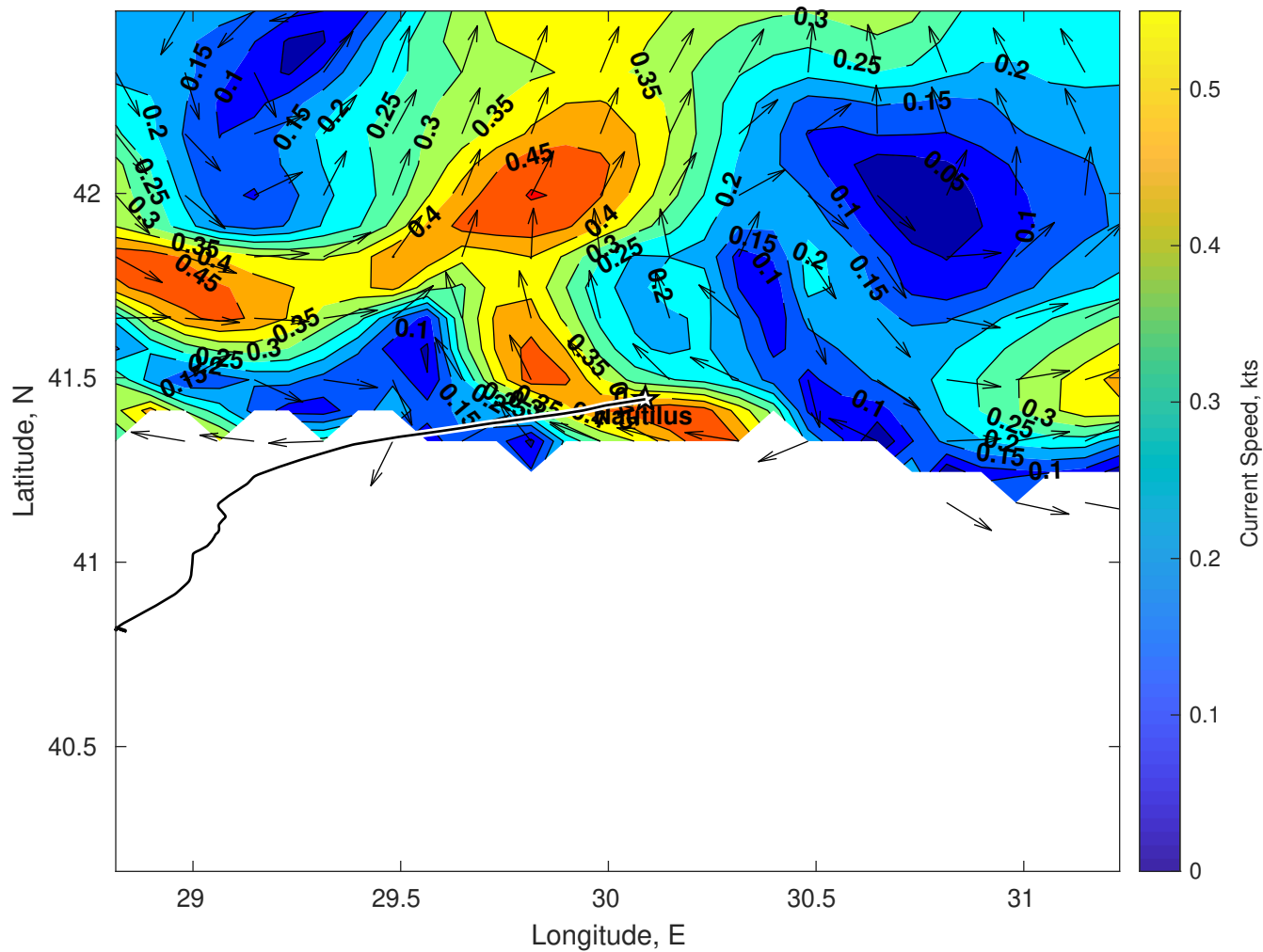
Surface Currents for Nautilus at 03-Nov-2025 00:00:00
