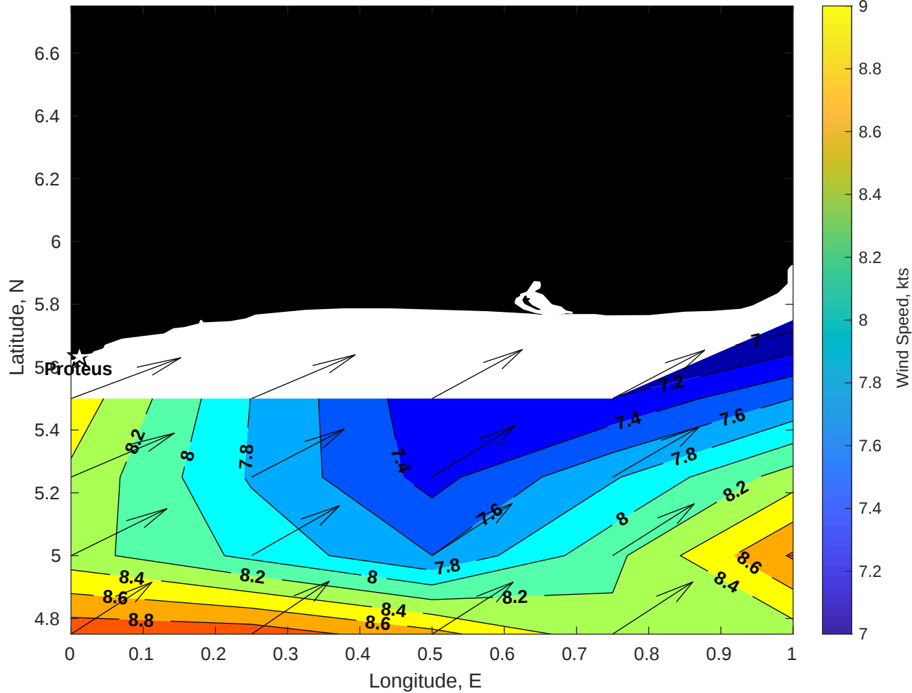
Winds (kts) for Proteus at 04-Nov-2025 09:00:00
