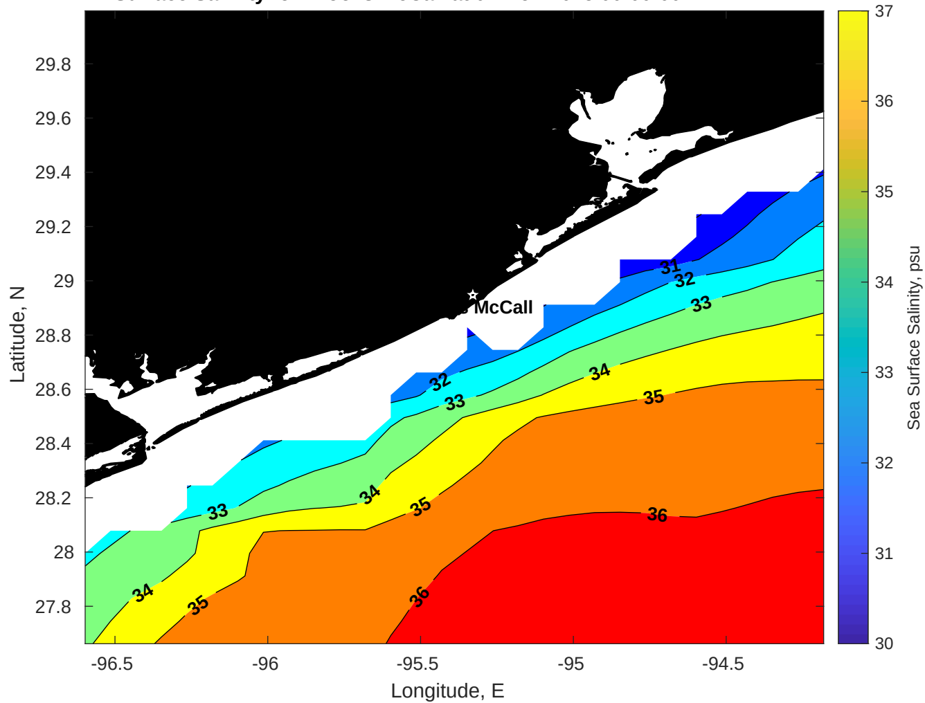
Surface Salinity for Brooks McCall at 04-Nov-2025 00:00:00
