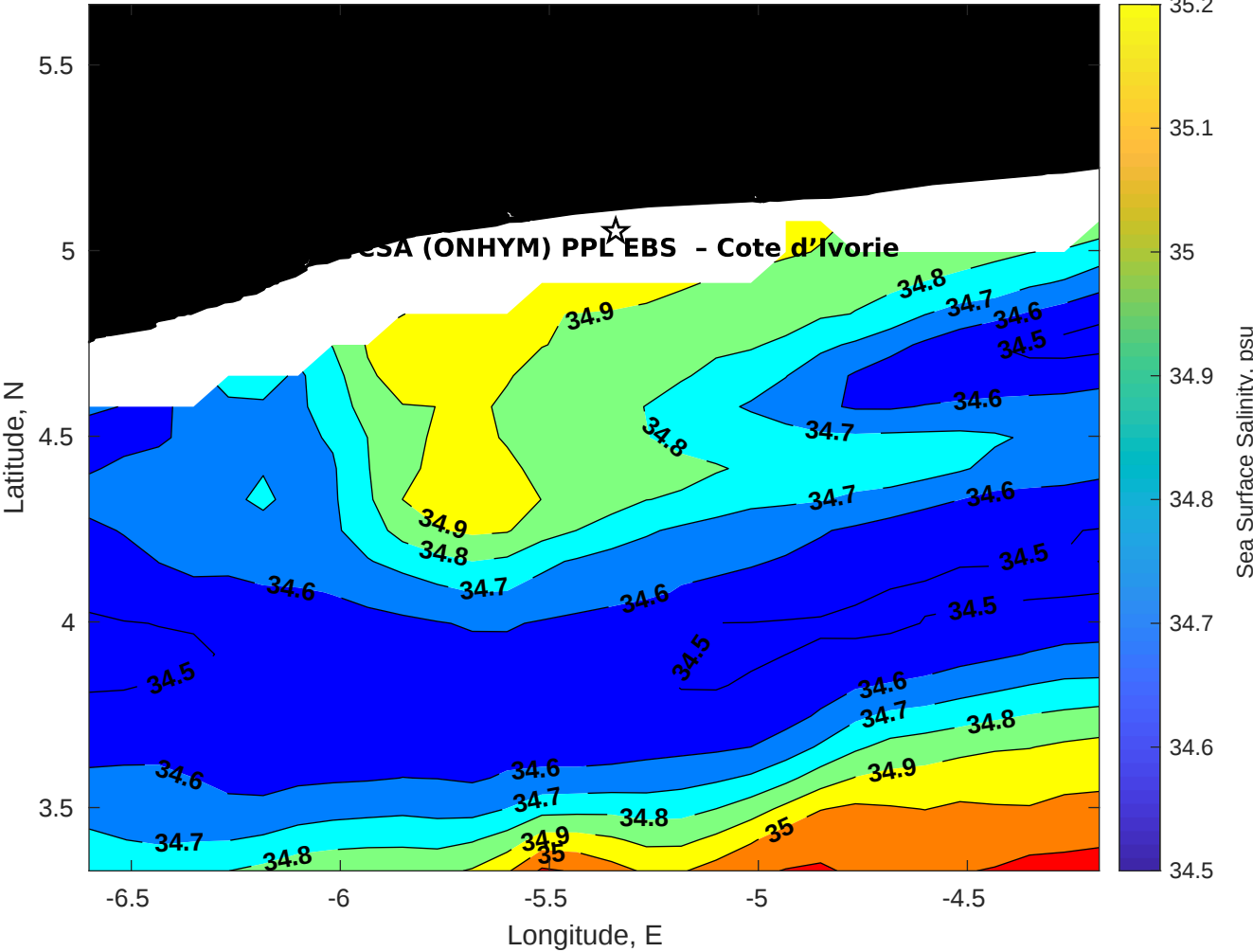
Surface Salinity for CSA (ONHYM) PPL EBS - Cote d'Ivoire at 04-Nov-2025 00:00:00
