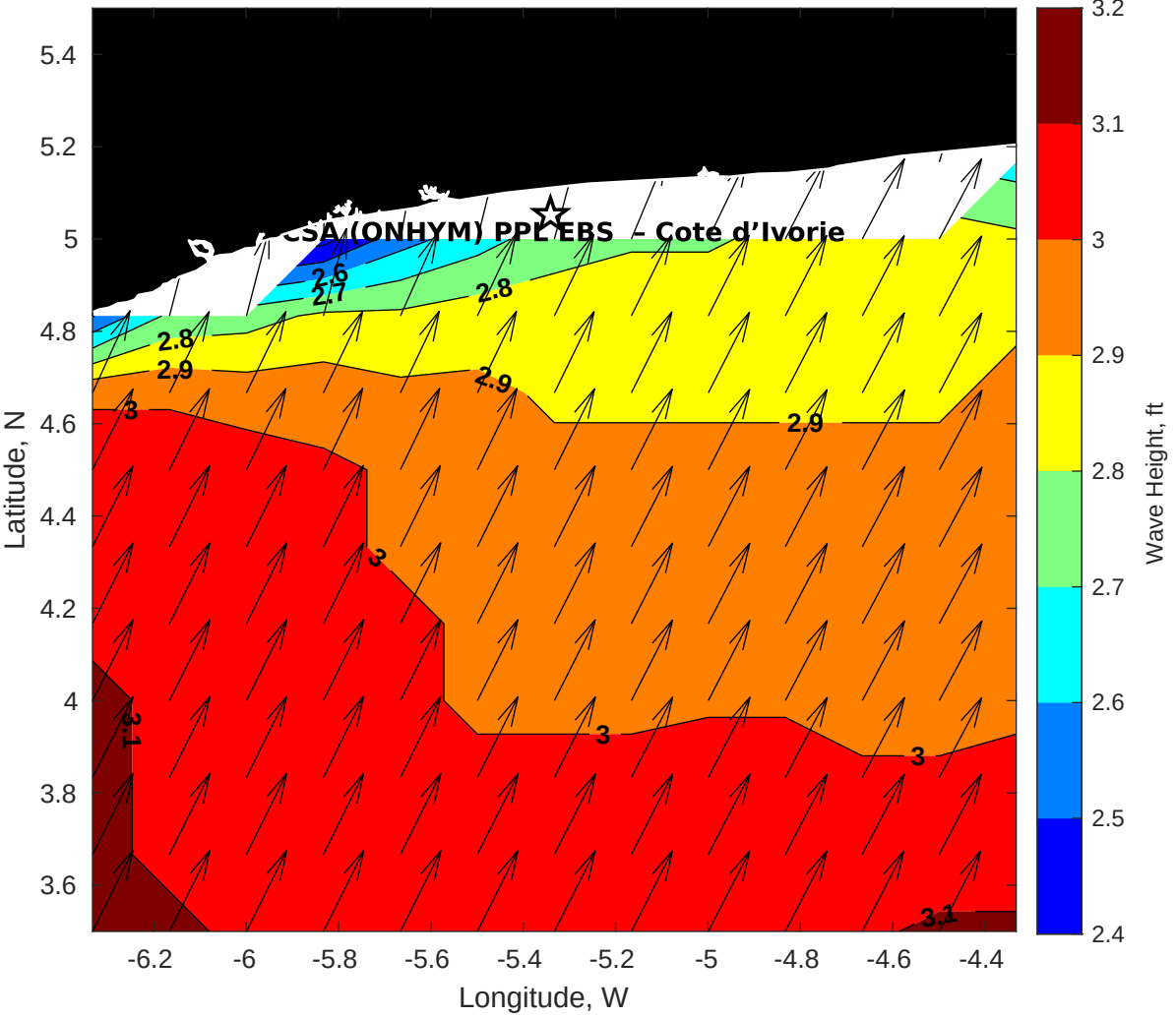
Wave Height (ft) for CSA (ONHYM) PPL EBS - Cote d'Ivoire at 05-Nov-2025 09:00:00
