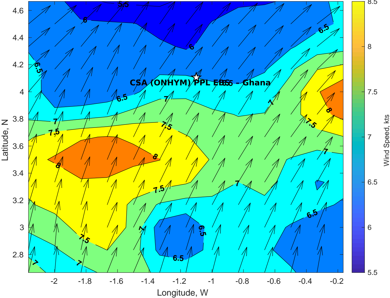
Winds (kts) for CSA (ONHYM) PPL EBS - Ghana at 05-Nov-2025 09:00:00
