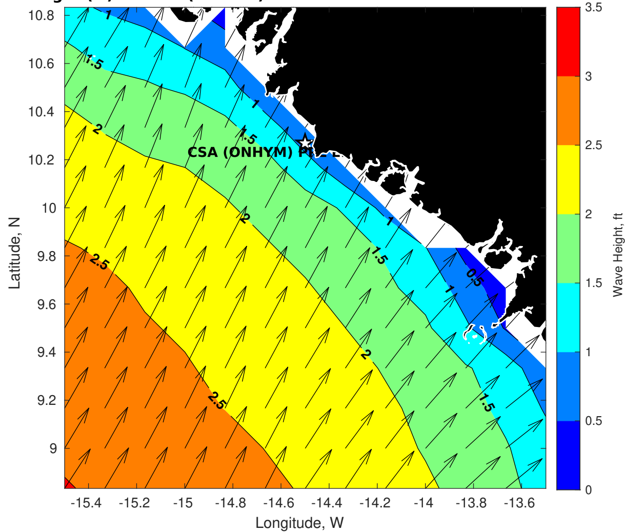
Wave Height (ft) for CSA (ONHYM) PPL EBS - Guinea at 05-Nov-2025 09:00:00
