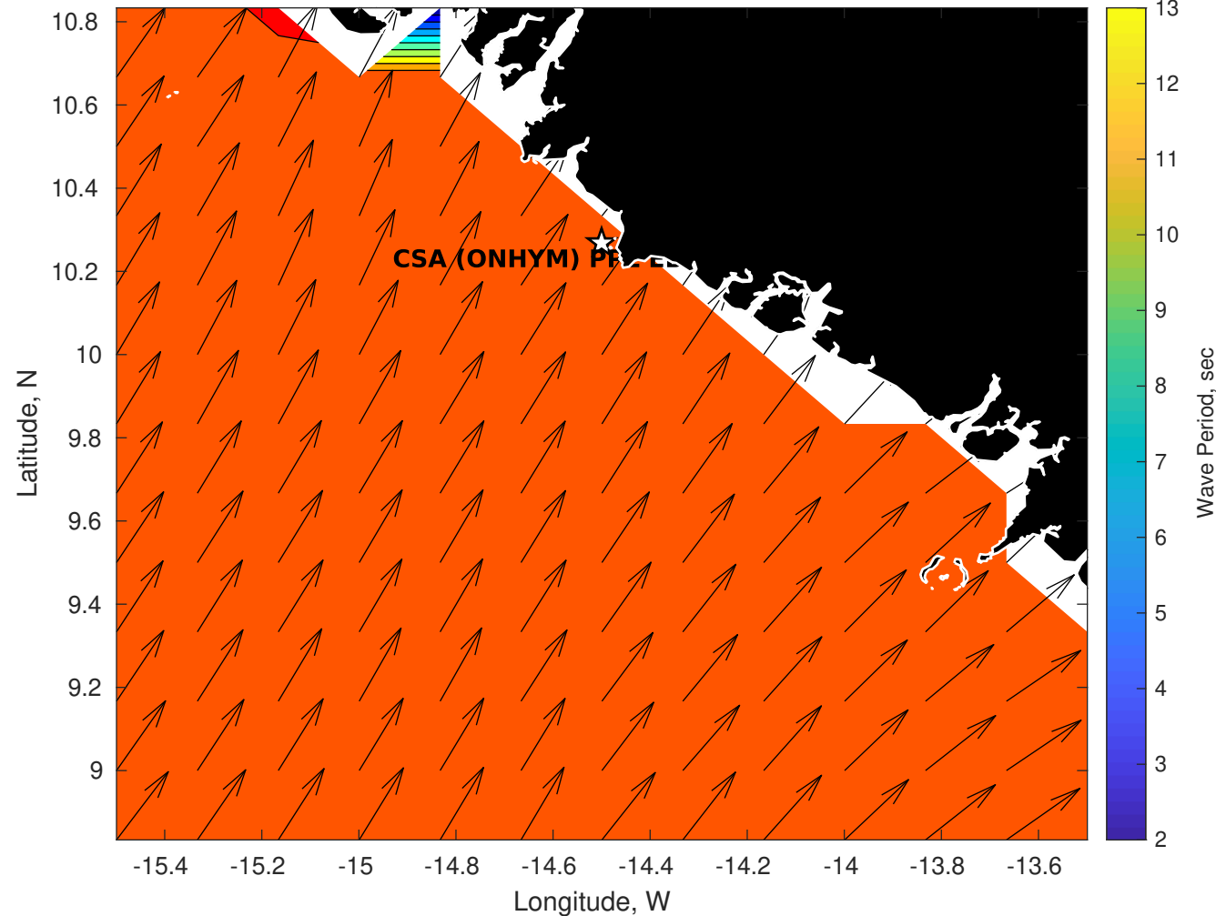
Wave Period (sec) for CSA (ONHYM) PPL EBS - Guinea at 05-Nov-2025 09:00:00
