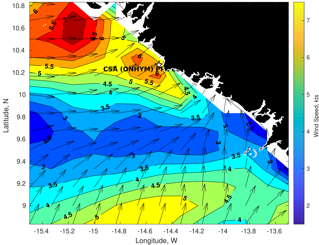
Winds (kts) for CSA (ONHYM) PPL EBS - Guinea at 05-Nov-2025 09:00:00
