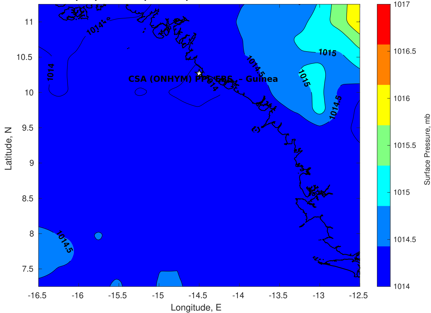
Surface Pressure (mb) for CSA (ONHYM) PPL EBS - Guinea at 05-Nov-2025 00:00:00
