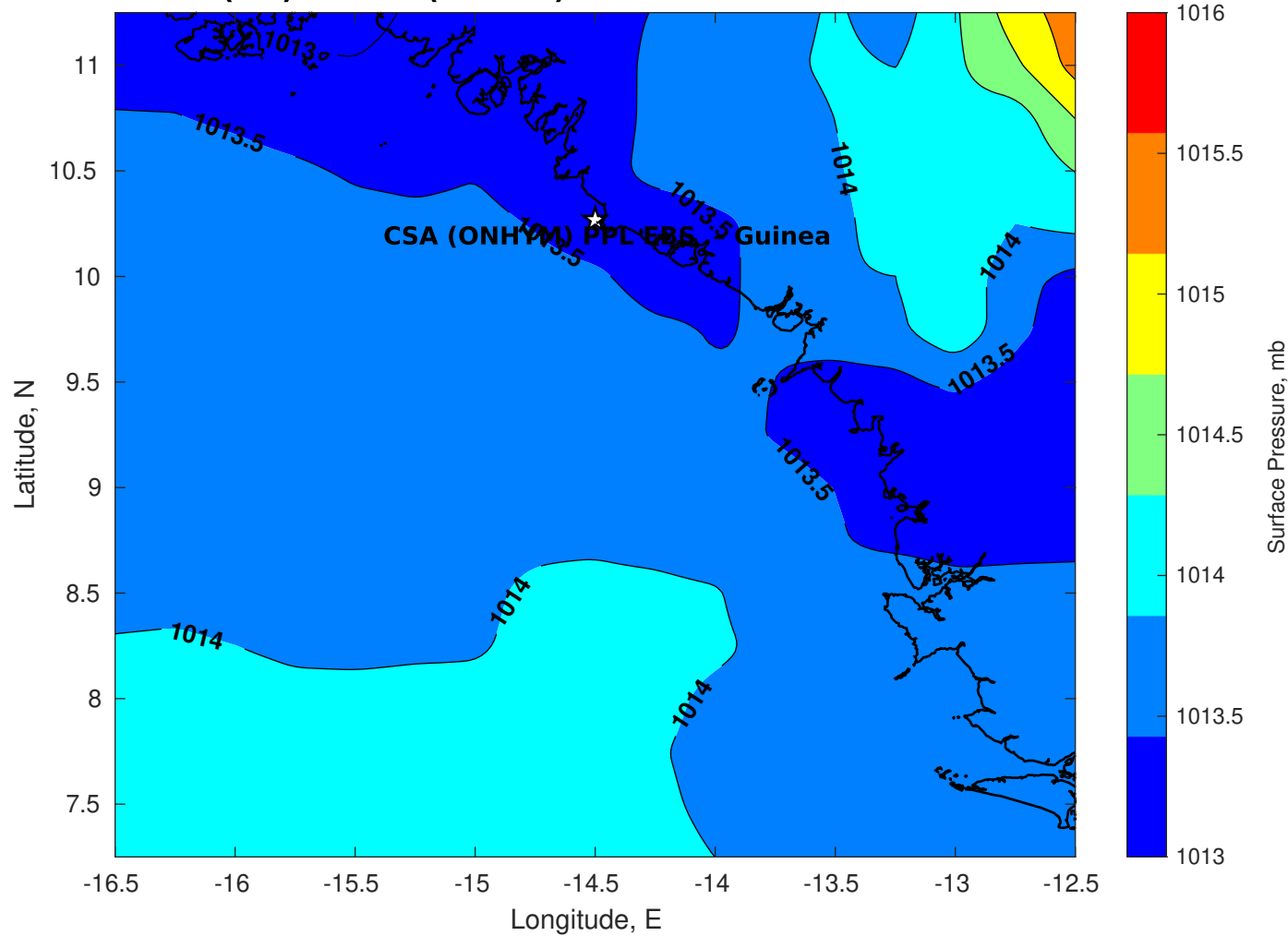
Surface Pressure (mb) for CSA (ONHYM) PPL EBS - Guinea at 06-Nov-2025 00:00:00
