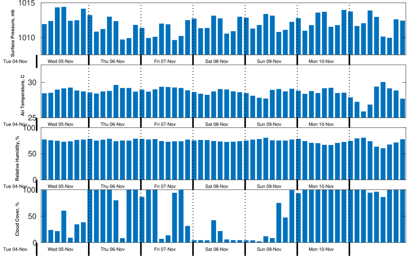
Met Forecast for CSA (ONHYM) PPL EBS - Guinea from 05-Nov-2025 00:00:00 to 12-Nov-2025 00:00:00
