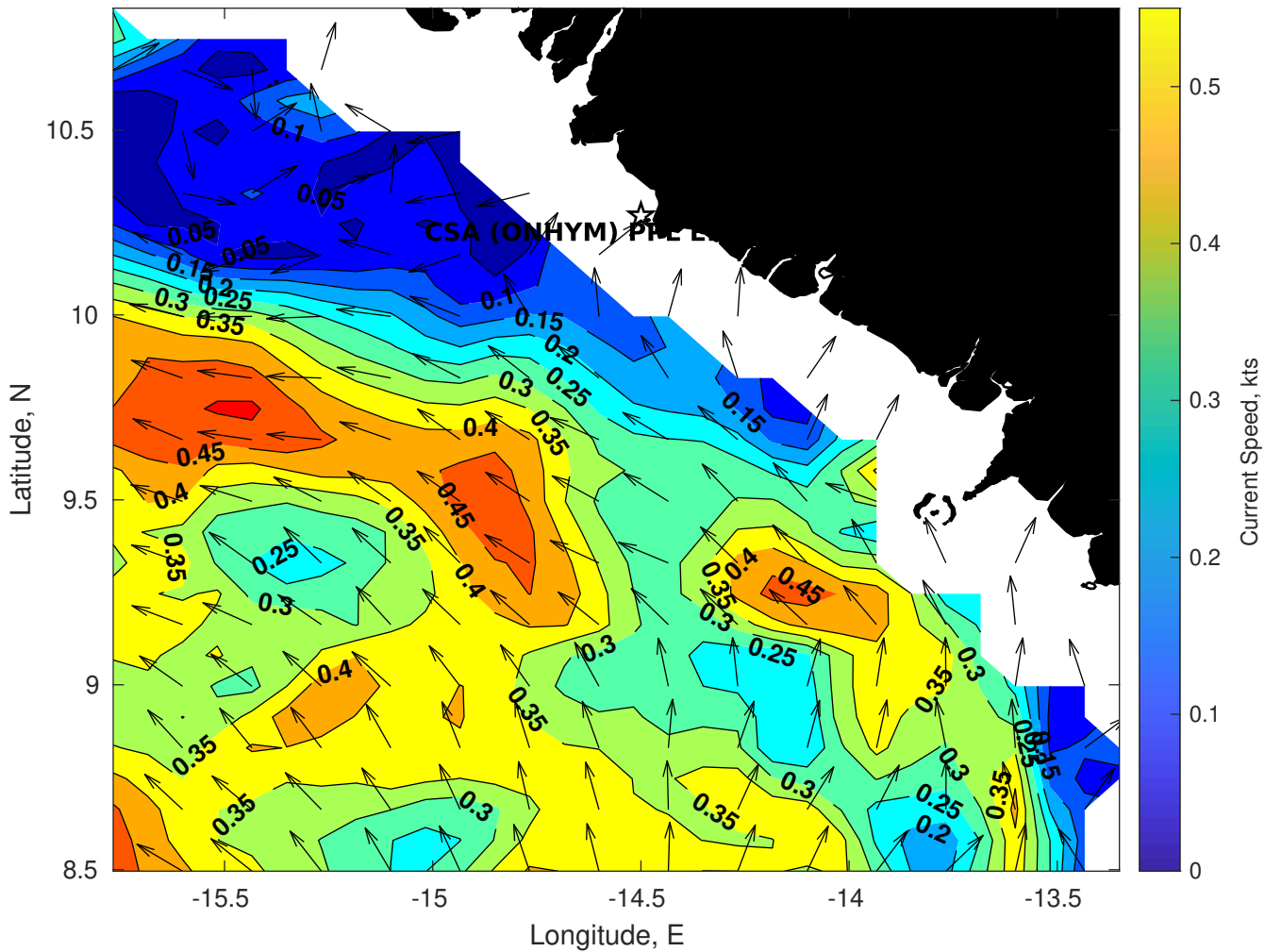
Surface Currents for CSA (ONHYM) PPL EBS - Guinea at 04-Nov-2025 00:00:00
