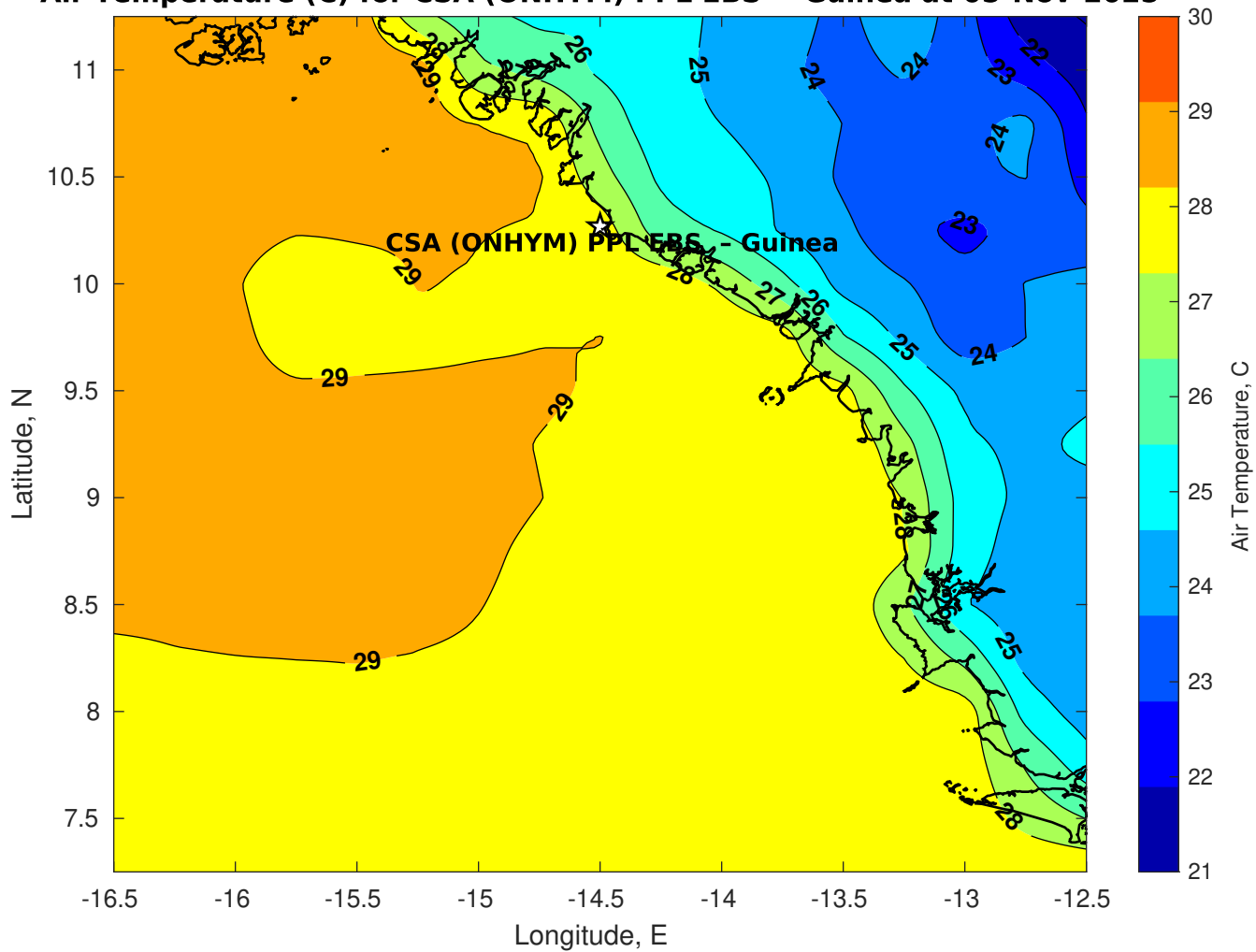
Air Temperature (C) for CSA (ONHYM) PPL EBS - Guinea at 05-Nov-2025
