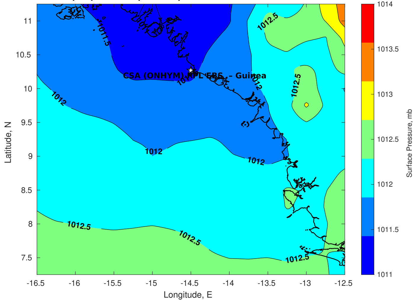
Surface Pressure (mb) for CSA (ONHYM) PPL EBS - Guinea at 07-Nov-2025 00:00:00
