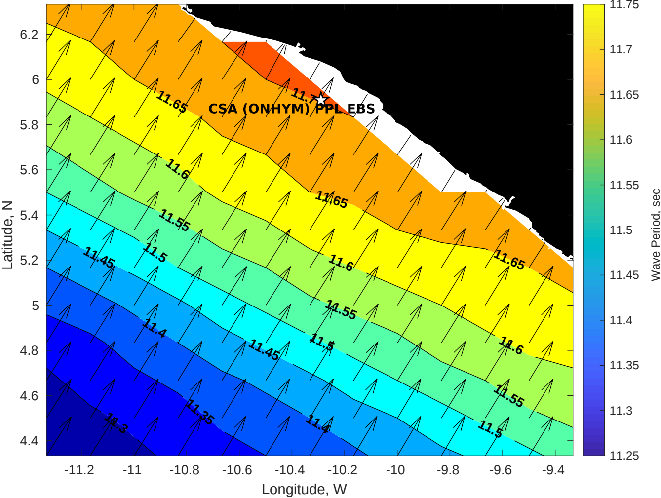
Wave Period (sec) for CSA (ONHYM) PPL EBS - Liberia at 05-Nov-2025 09:00:00
