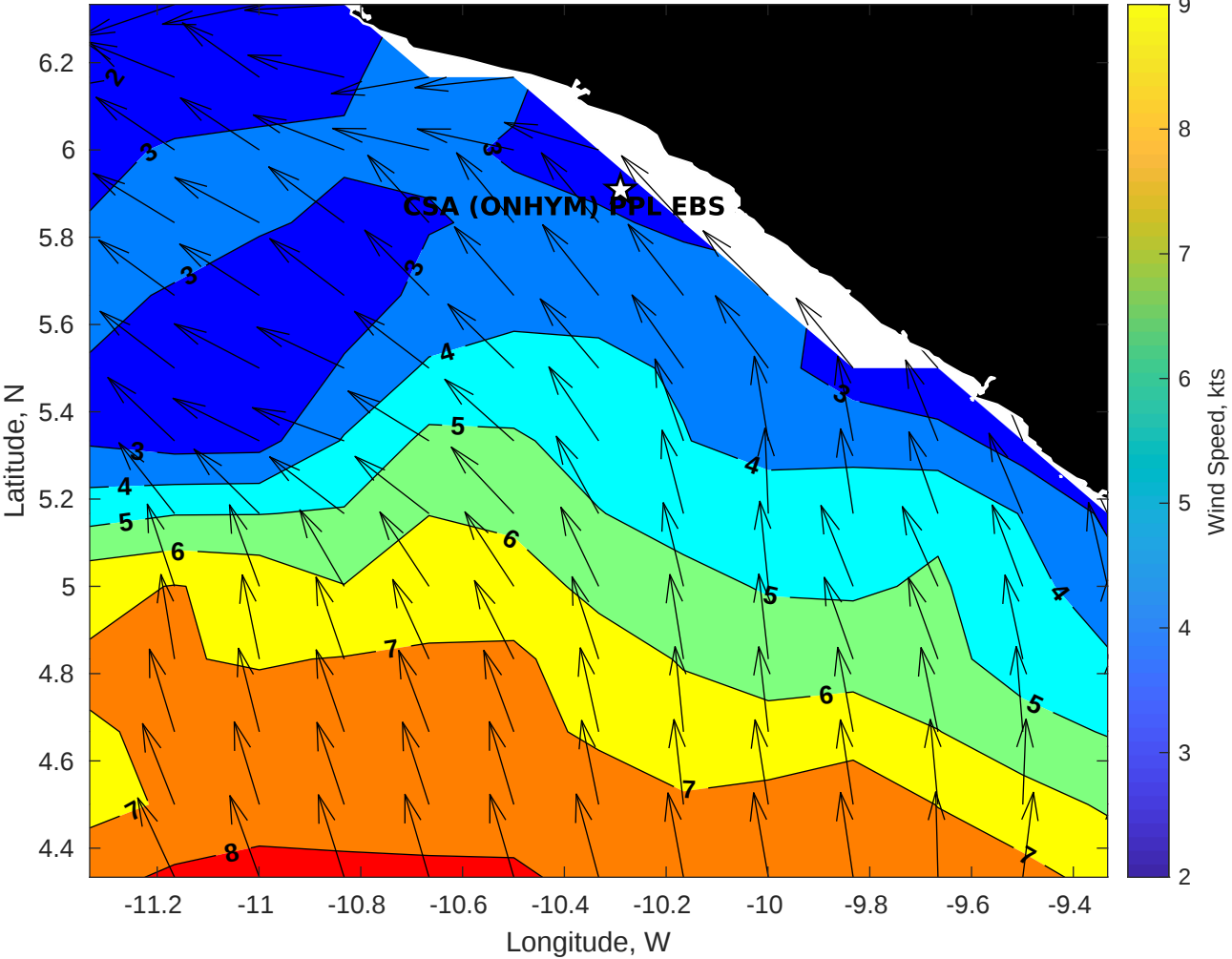
Winds (kts) for CSA (ONHYM) PPL EBS - Liberia at 05-Nov-2025 09:00:00
