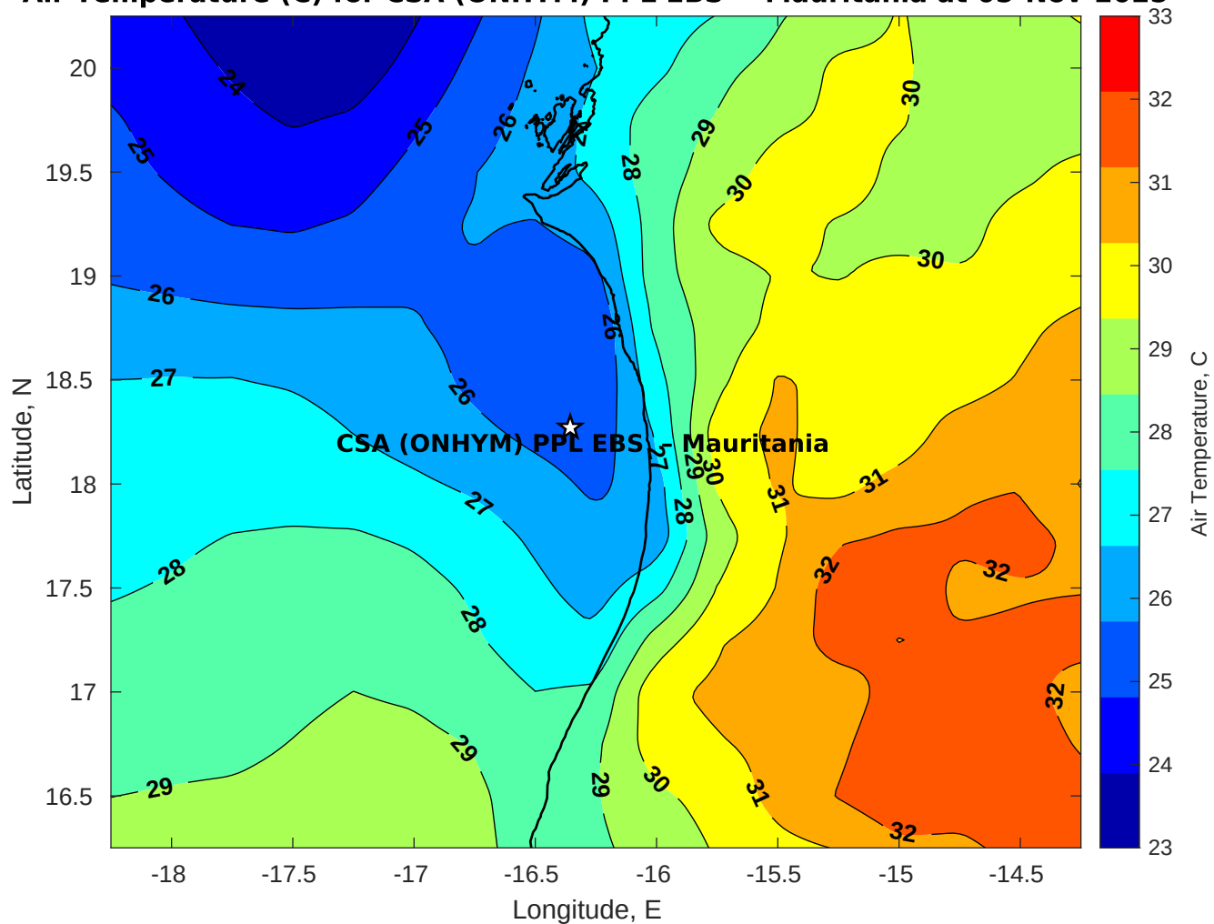
Air Temperature (C) for CSA (ONHYM) PPL EBS - Mauritania at 05-Nov-2025
