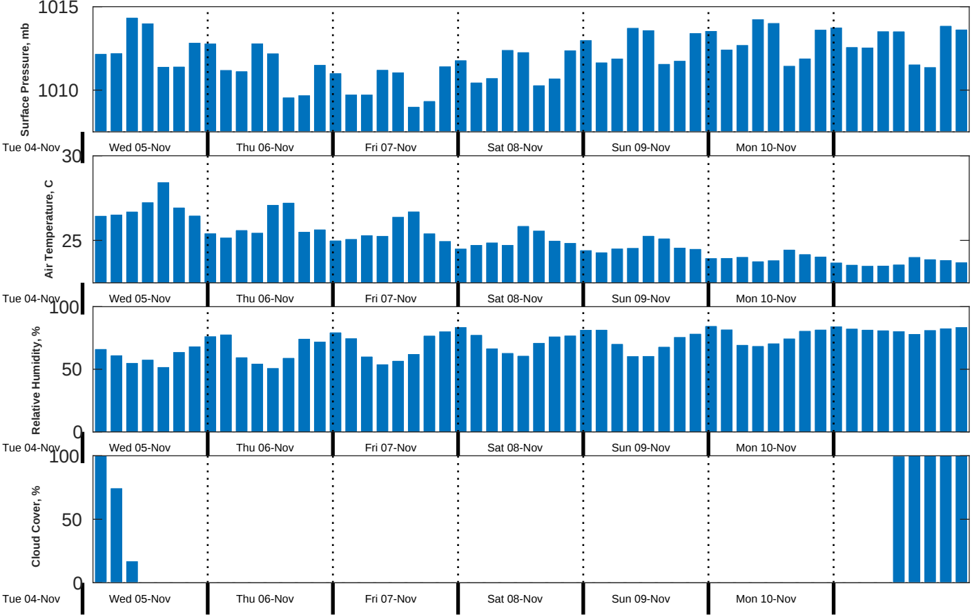
Met Forecast for CSA (ONHYM) PPL EBS - Mauritania from 05-Nov-2025 00:00:00 to 12-Nov-2025 00:00:00
