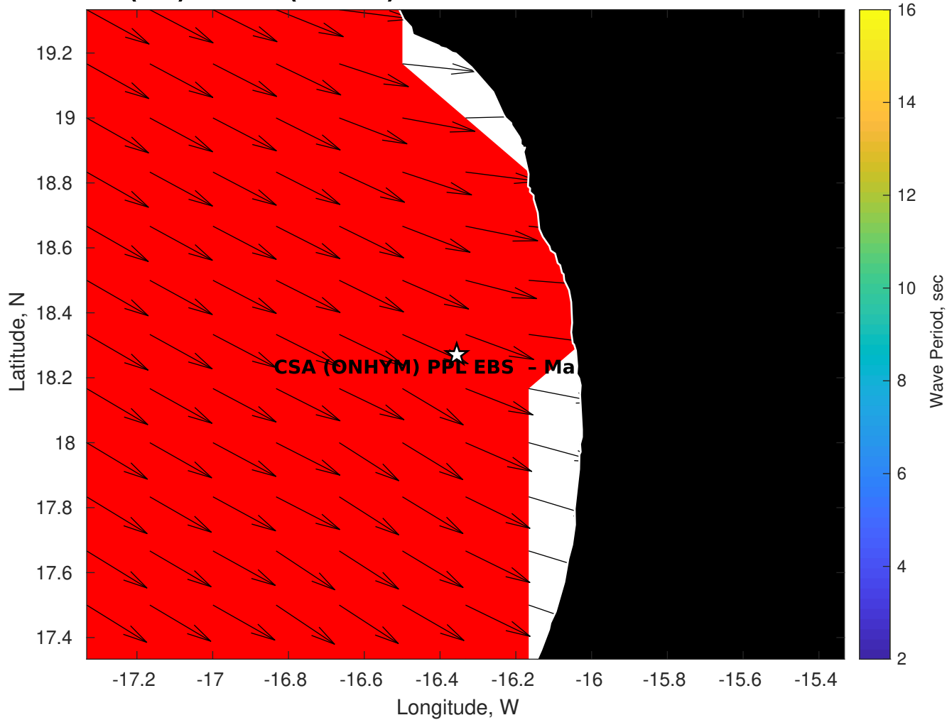
Wave Period (sec) for CSA (ONHYM) PPL EBS - Mauritania at 05-Nov-2025 09:00:00
