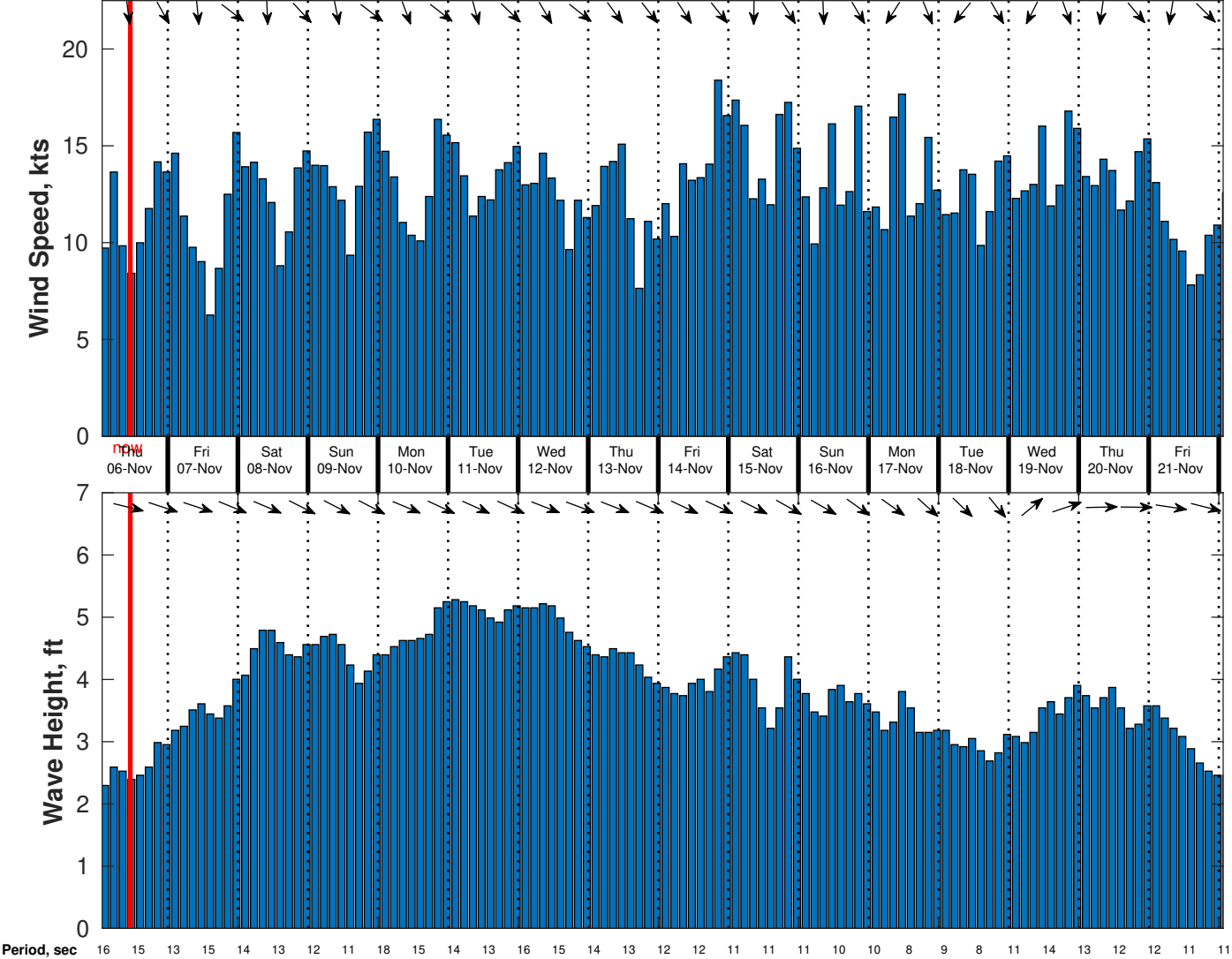
Wind & Wave Forecast for CSA (ONHYM) PPL EBS - Mauritania from 05-Nov-2025 01:00:00 to 21-Nov-2025 01:00:00
