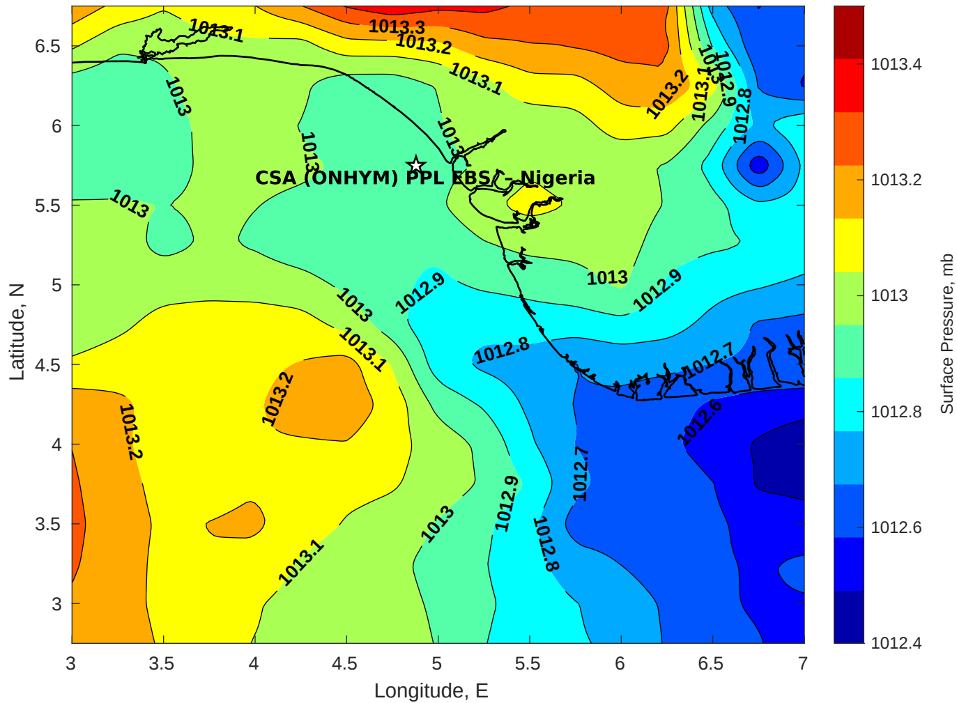
Surface Pressure (mb) for CSA (ONHYM) PPL EBS - Nigeria at 05-Nov-2025 00:00:00
