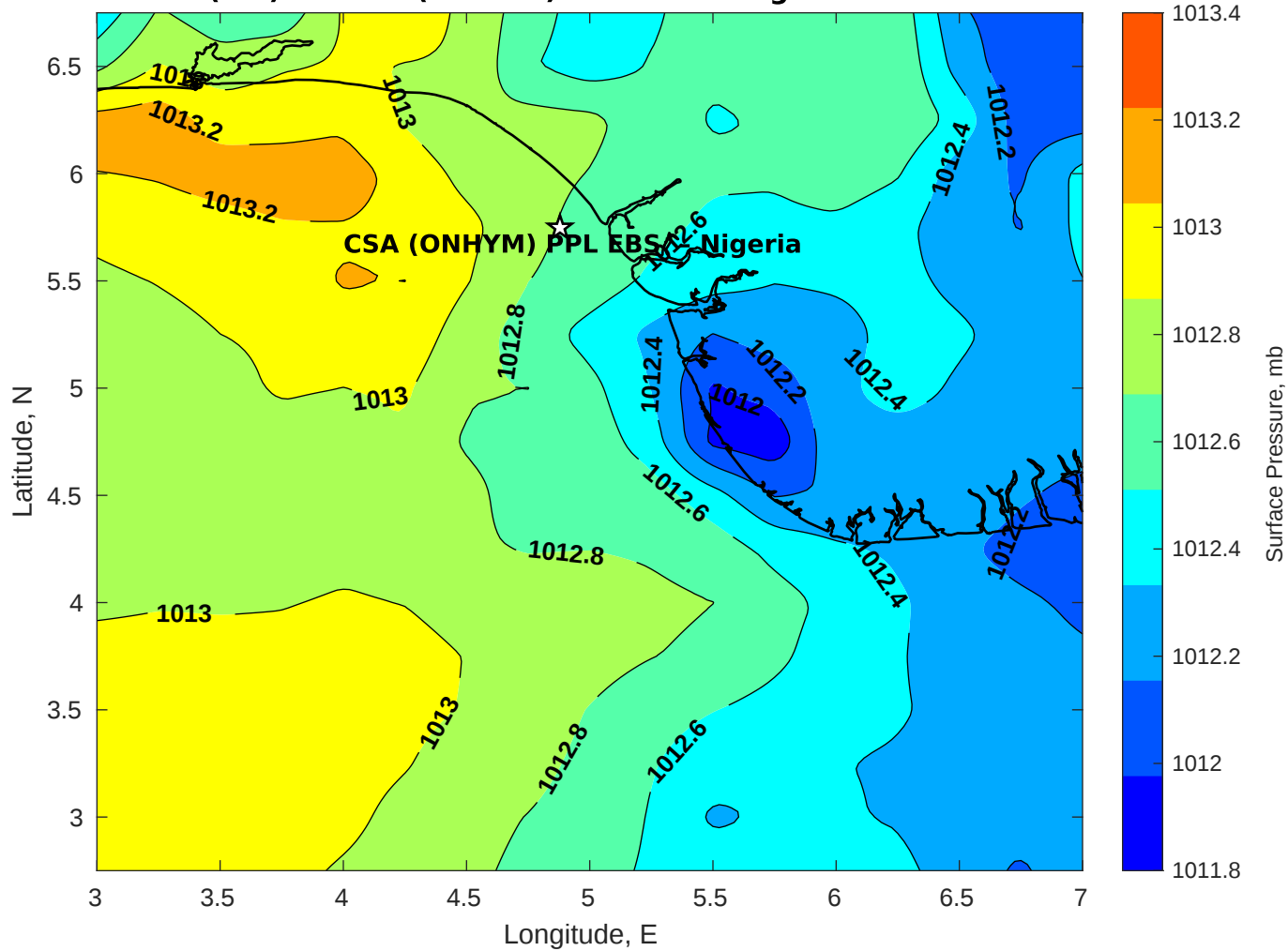
Surface Pressure (mb) for CSA (ONHYM) PPL EBS - Nigeria at 06-Nov-2025 00:00:00
