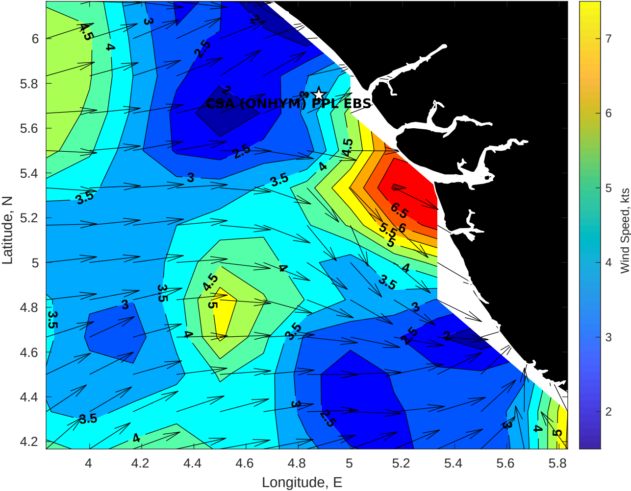
Winds (kts) for CSA (ONHYM) PPL EBS - Nigeria at 05-Nov-2025 09:00:00
