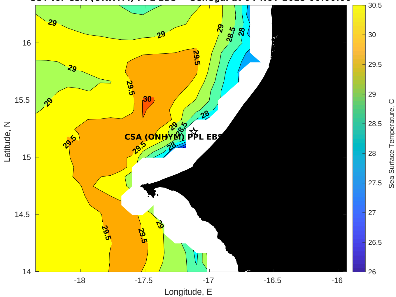
SST for CSA (ONHYM) PPL EBS - Senegal at 04-Nov-2025 00:00:00
