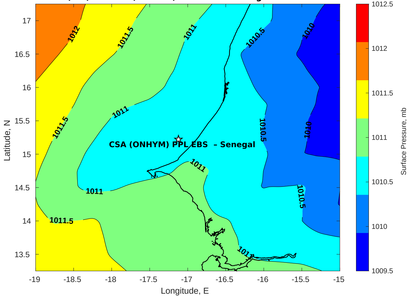
Surface Pressure (mb) for CSA (ONHYM) PPL EBS - Senegal at 07-Nov-2025 00:00:00
