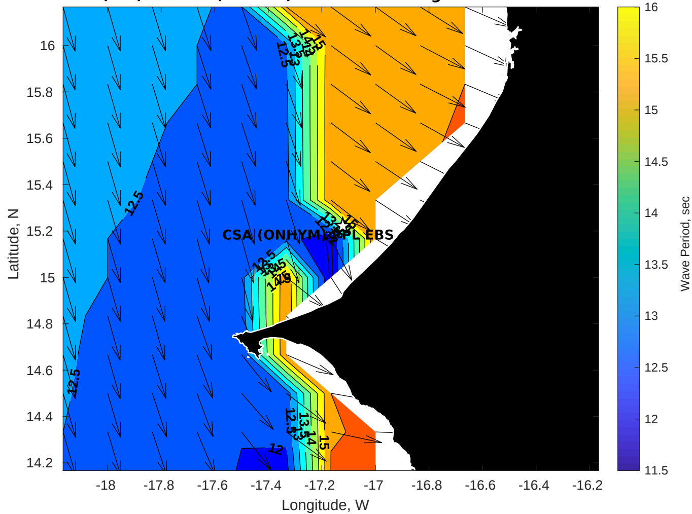
Wave Period (sec) for CSA (ONHYM) PPL EBS - Senegal at 05-Nov-2025 09:00:00
