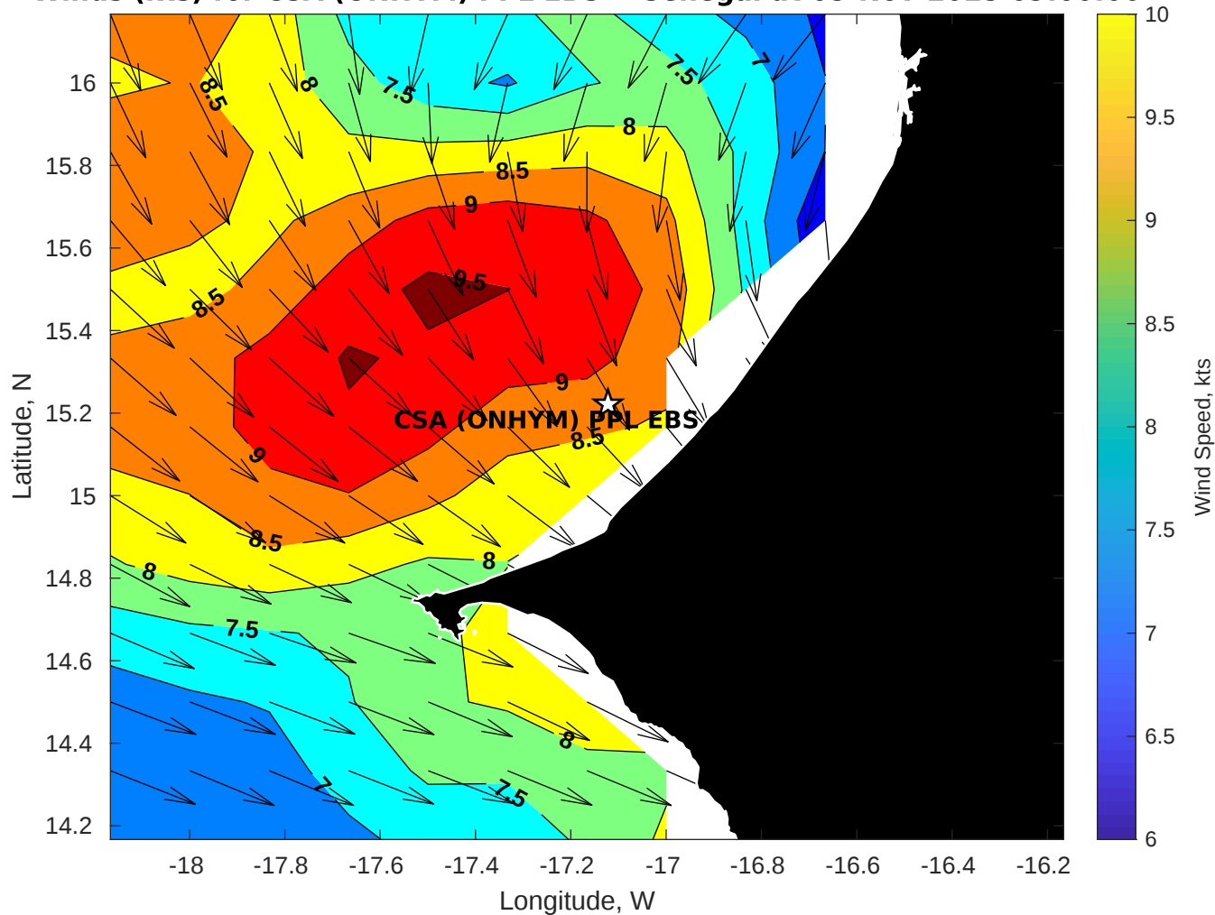
Winds (kts) for CSA (ONHYM) PPL EBS - Senegal at 05-Nov-2025 09:00:00
