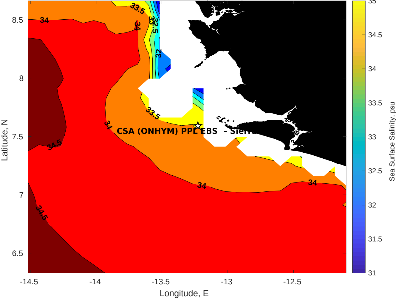
Surface Salinity for CSA (ONHYM) PPL EBS - Sierra Leone at 04-Nov-2025 00:00:00
