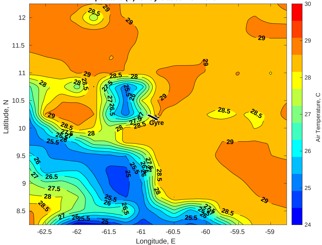
Air Temperature (C) for Gyre at 05-Nov-2025
