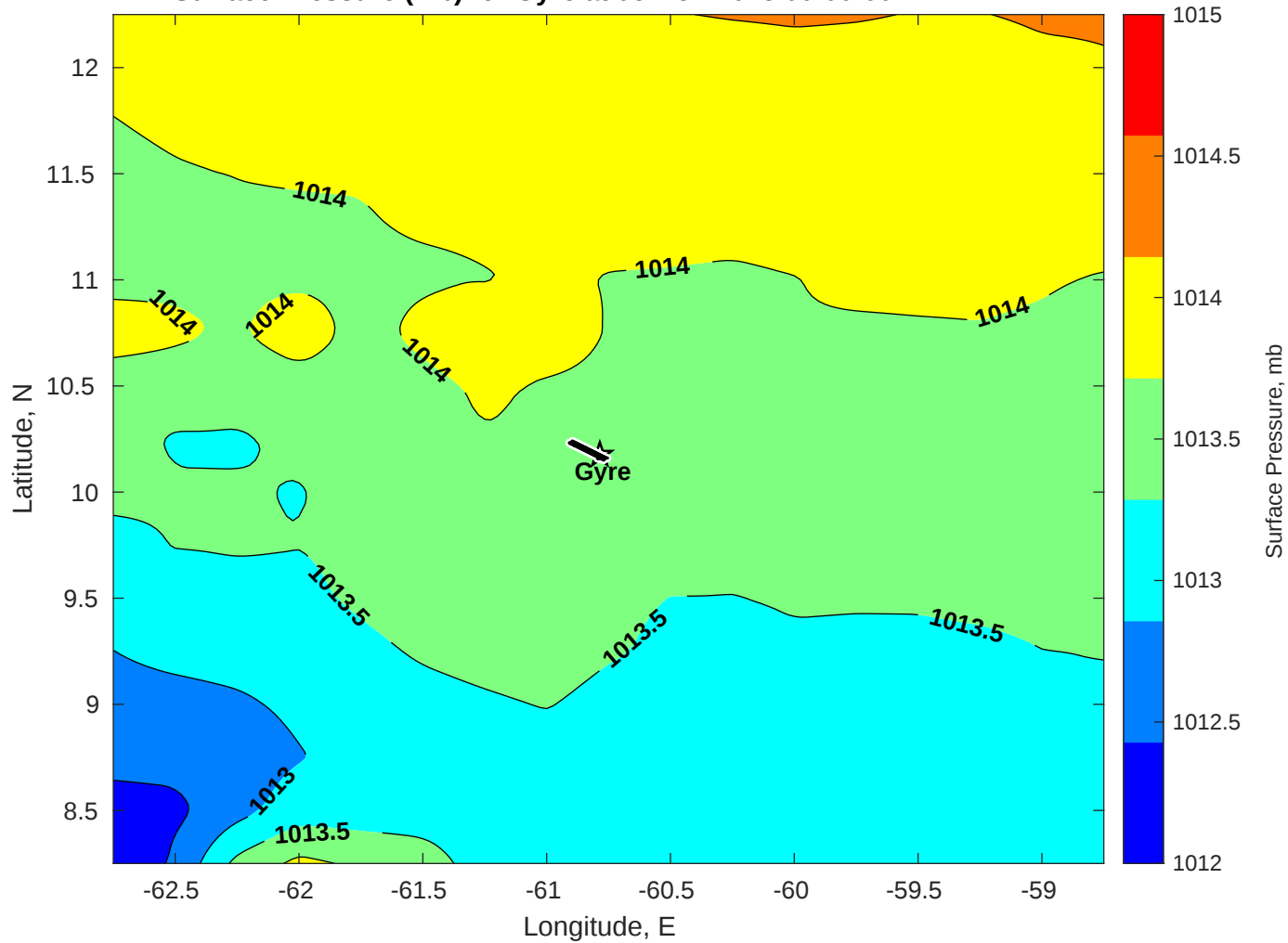
Surface Pressure (mb) for Gyre at 06-Nov-2025 00:00:00
