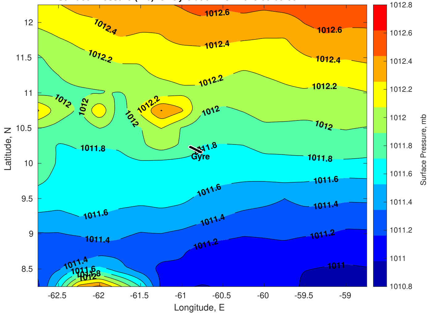
Surface Pressure (mb) for Gyre at 07-Nov-2025 00:00:00
