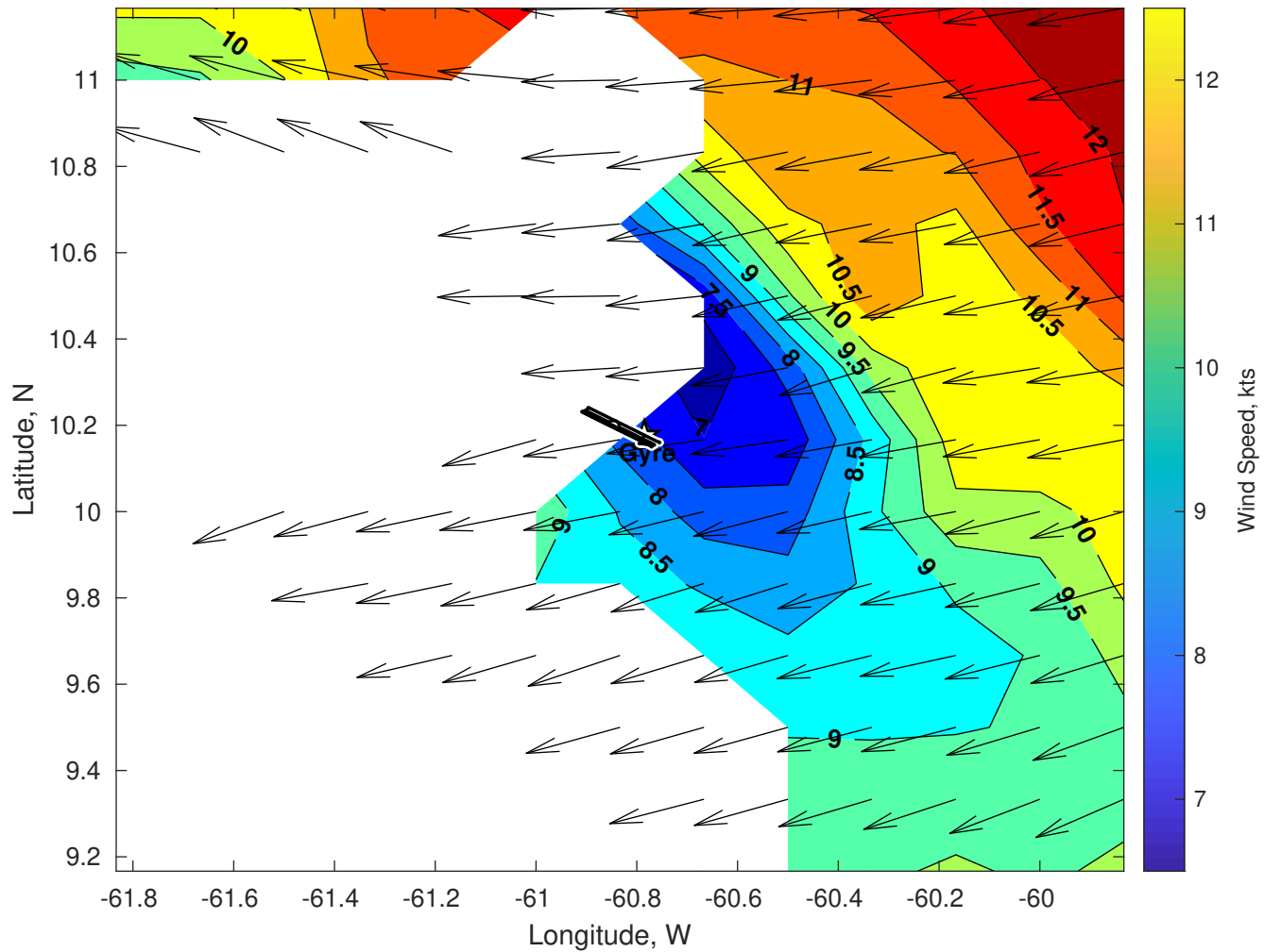
Winds (kts) for Gyre at 05-Nov-2025 09:00:00
