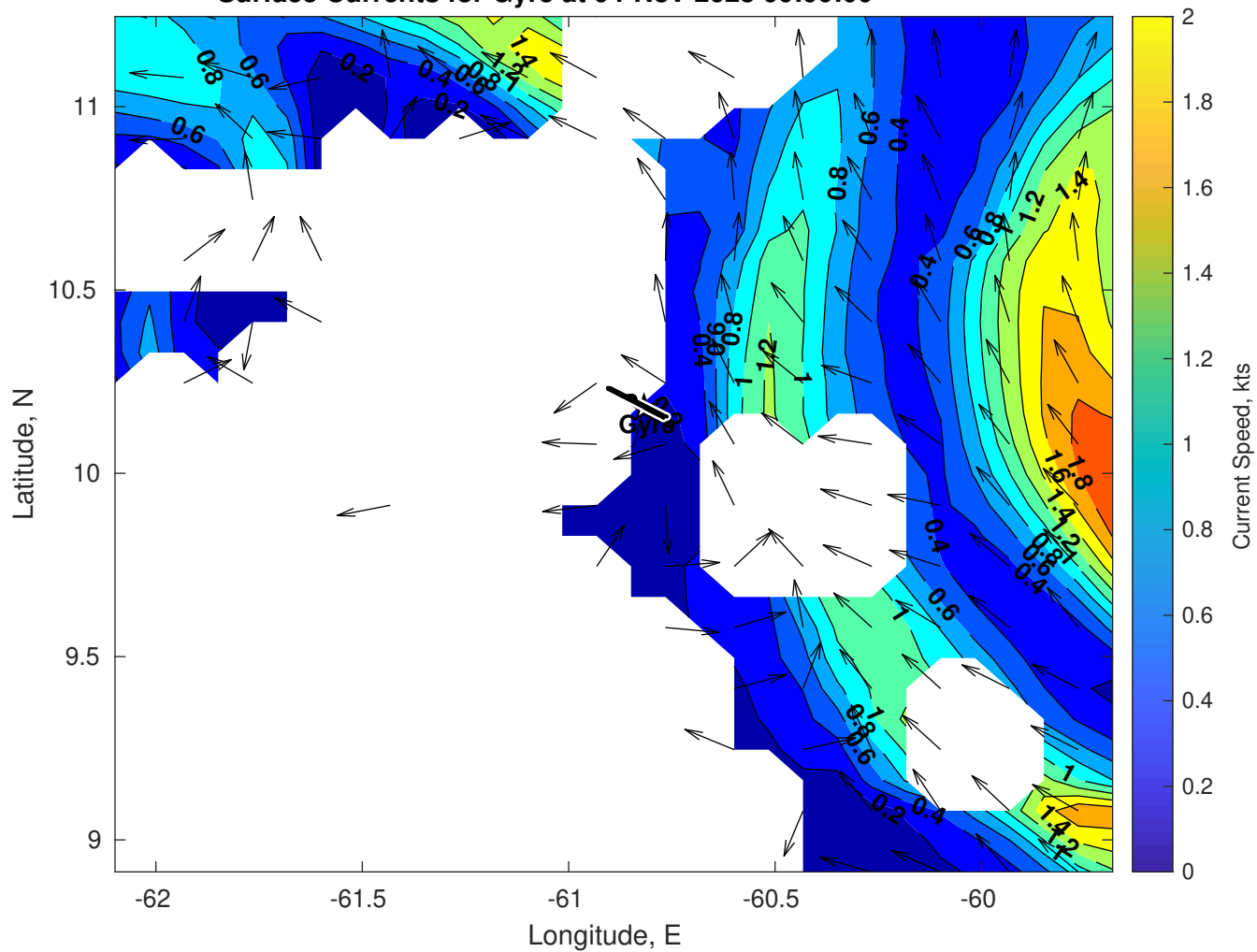
Surface Currents for Gyre at 04-Nov-2025 00:00:00
