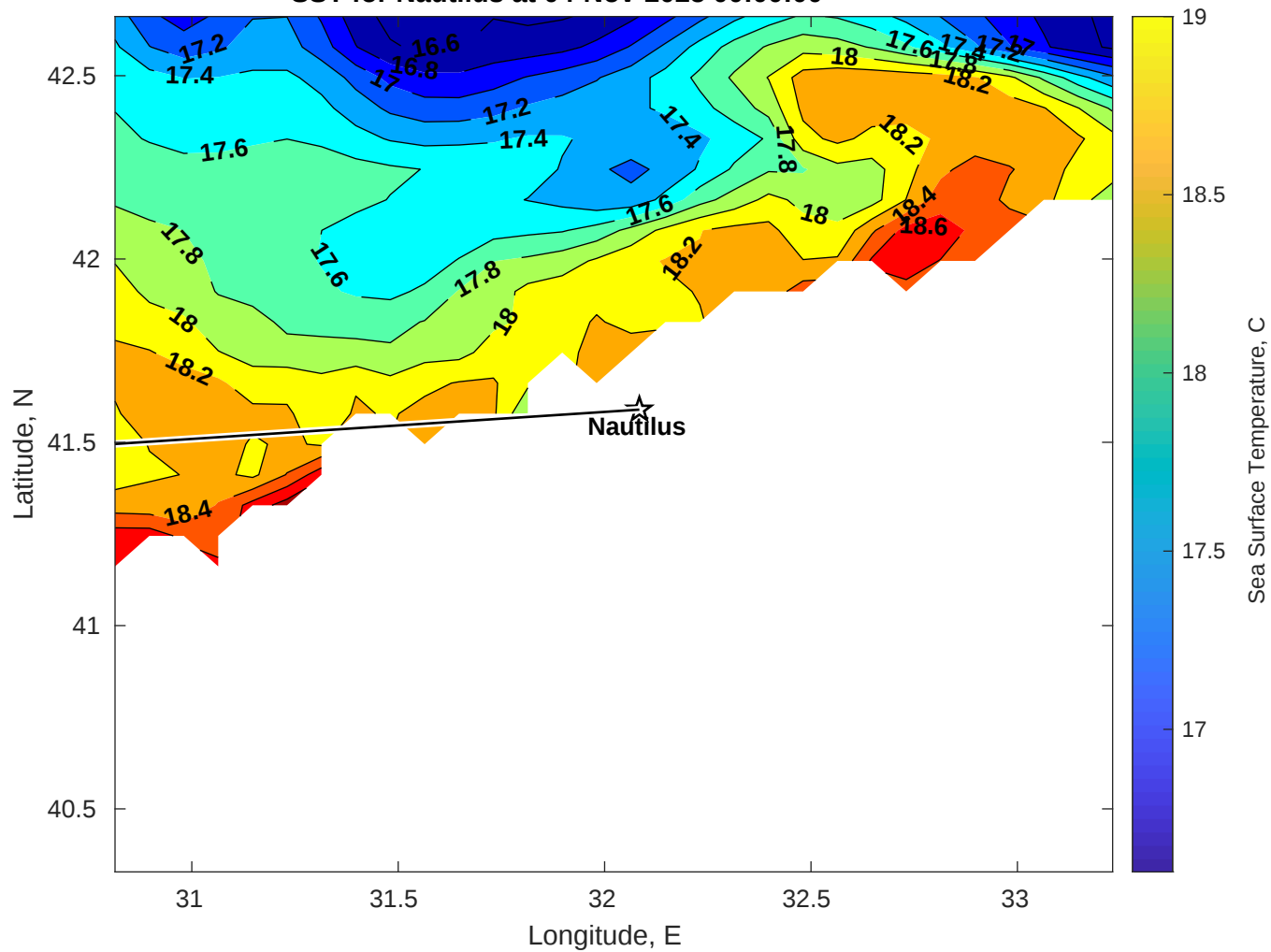
SST for Nautilus at 04-Nov-2025 00:00:00
