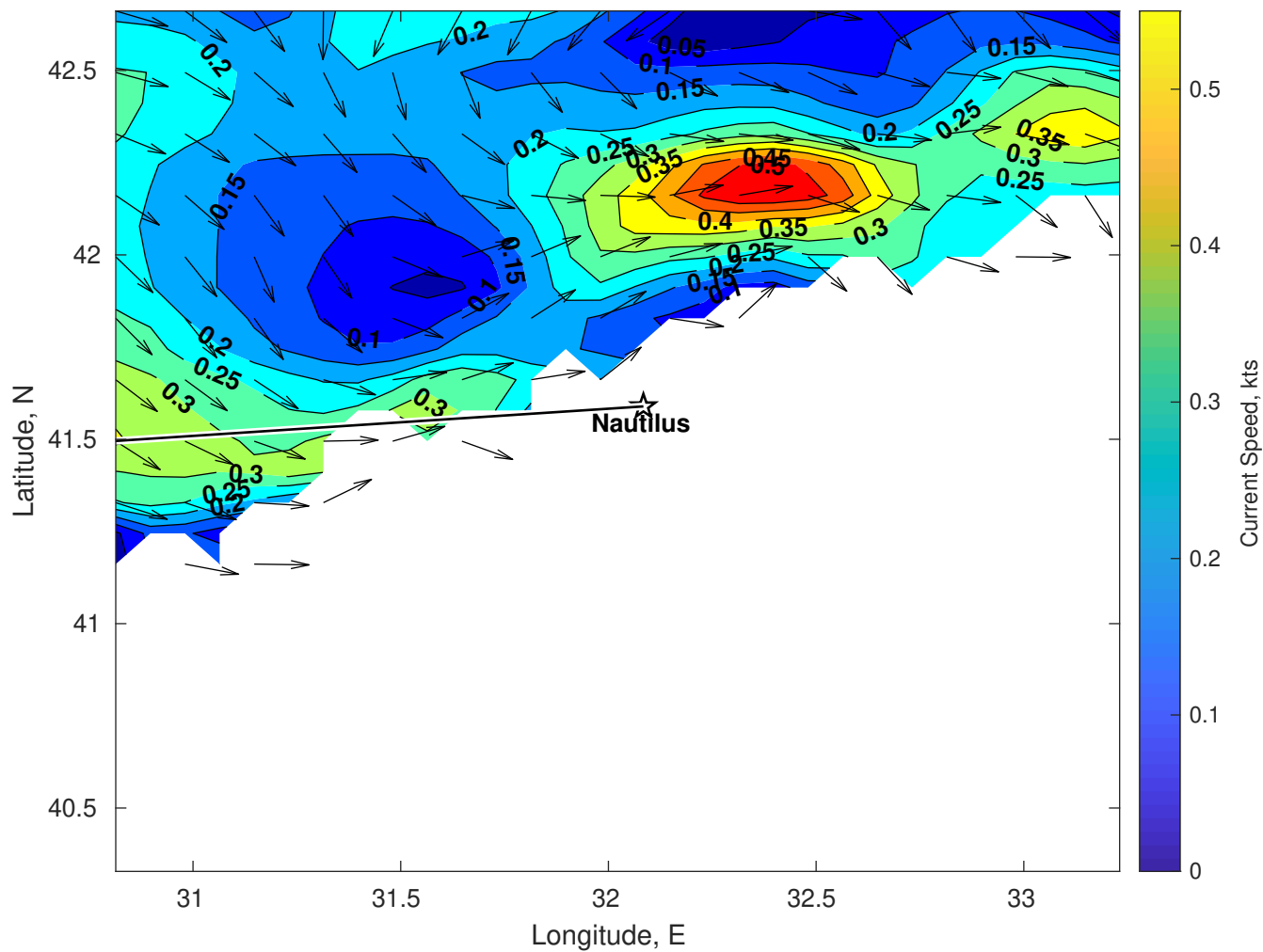
Surface Currents for Nautilus at 04-Nov-2025 00:00:00
