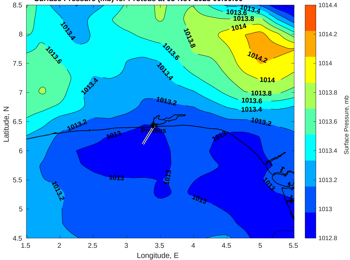
Surface Pressure (mb) for Proteus at 05-Nov-2025 00:00:00
