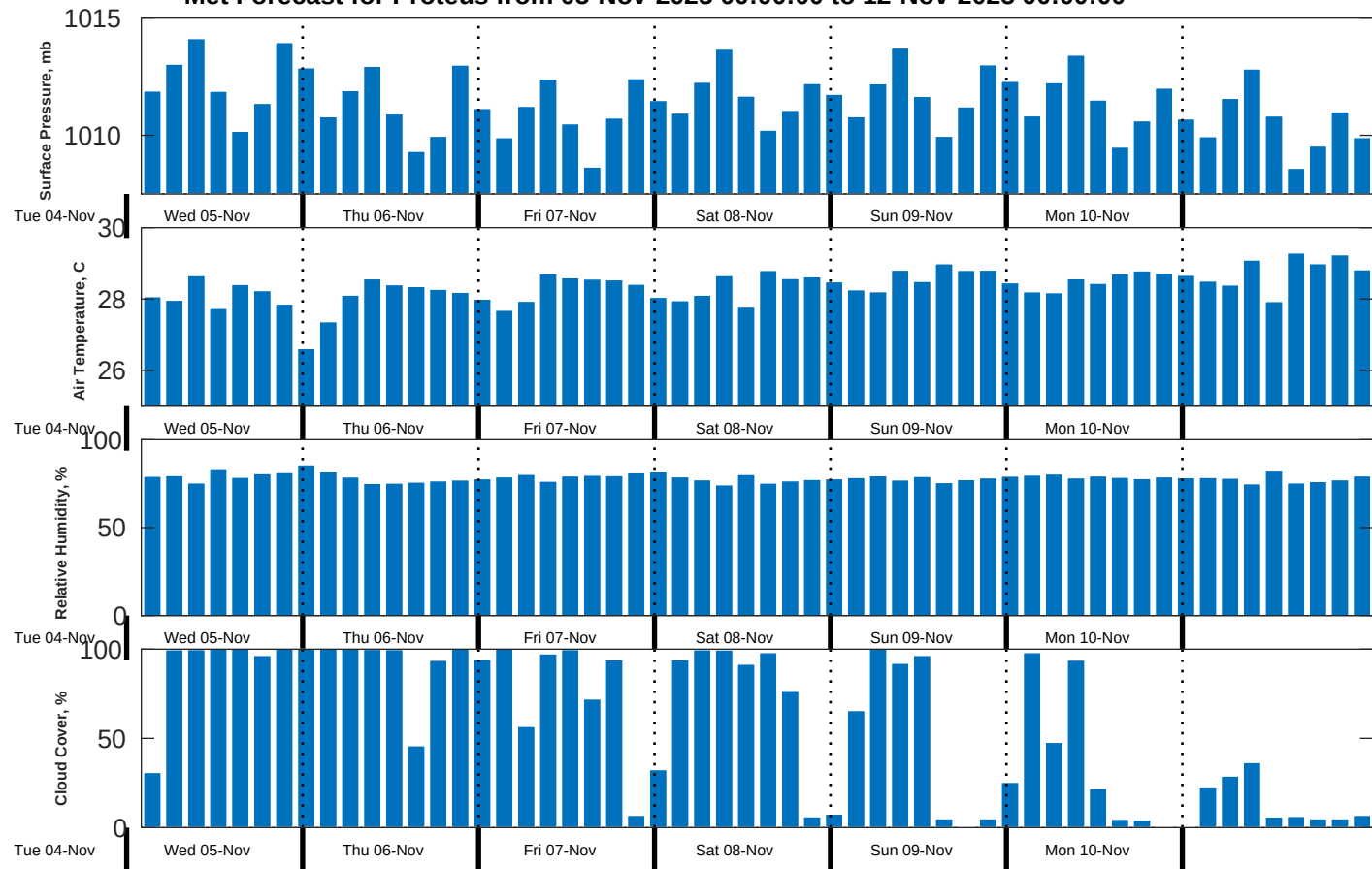
Met Forecast for Proteus from 05-Nov-2025 00:00:00 to 12-Nov-2025 00:00:00
