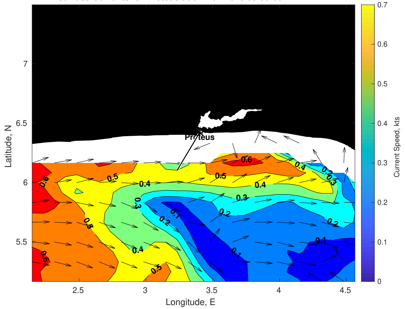
Surface Currents for Proteus at 04-Nov-2025 00:00:00
