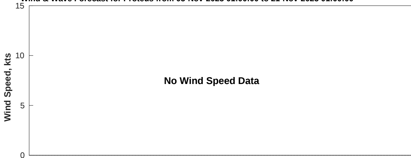
Wind & Wave Forecast for Proteus from 05-Nov-2025 01:00:00 to 21-Nov-2025 01:00:00
