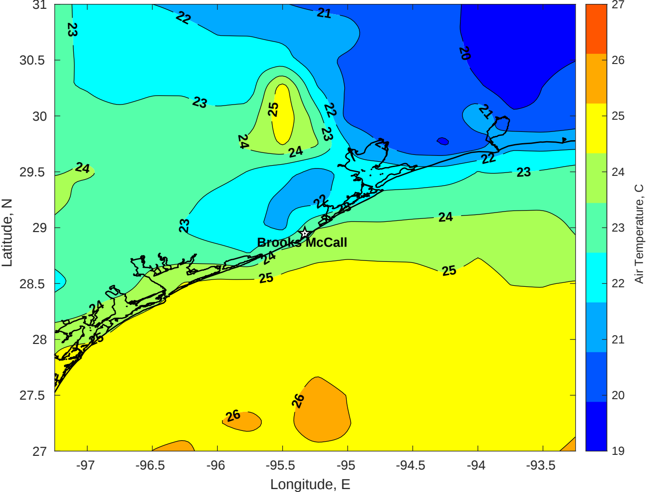
Air Temperature (C) for Brooks McCall at 06-Nov-2025
