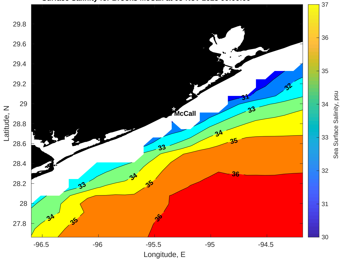
Surface Salinity for Brooks McCall at 05-Nov-2025 00:00:00
