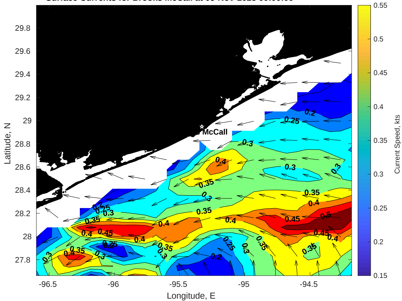
Surface Currents for Brooks McCall at 05-Nov-2025 00:00:00
