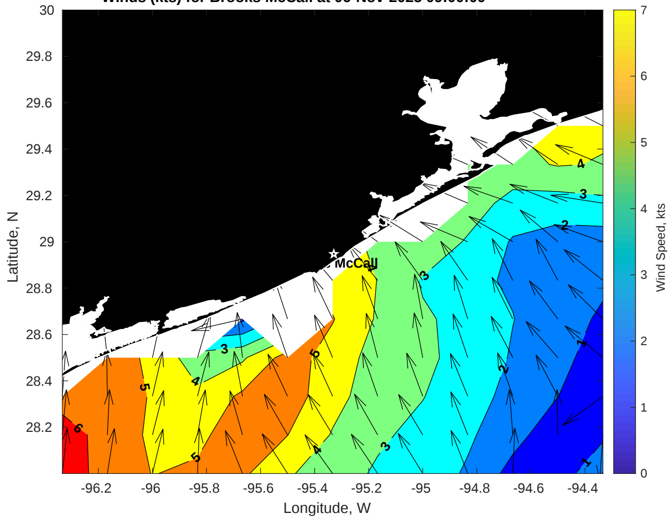
Winds (kts) for Brooks McCall at 06-Nov-2025 09:00:00
