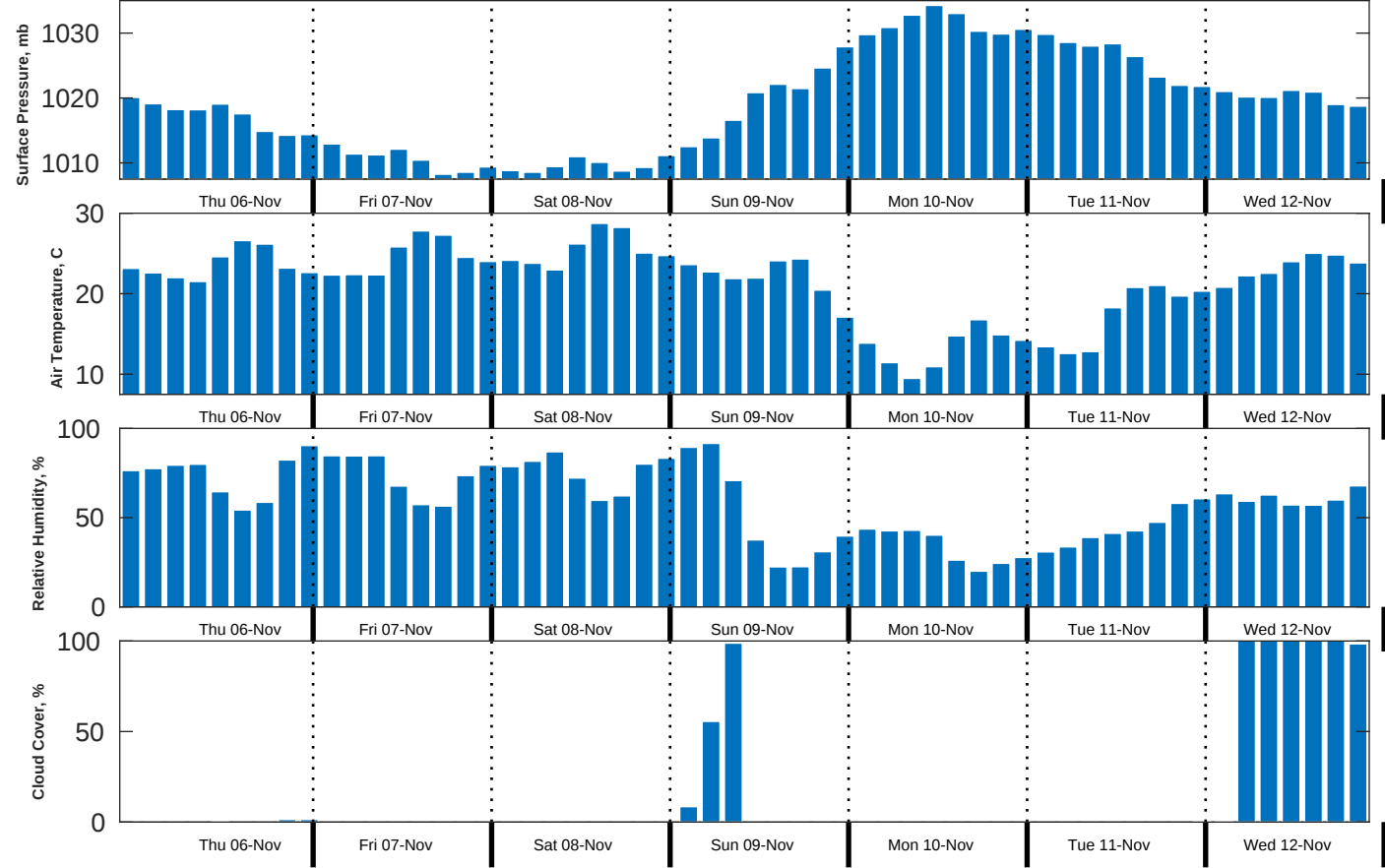
Met Forecast for Brooks McCall from 06-Nov-2025 00:00:00 to 13-Nov-2025 00:00:00
