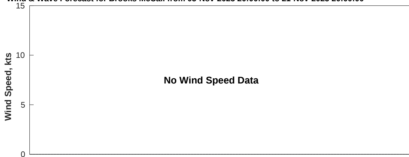
Wind & Wave Forecast for Brooks McCall from 05-Nov-2025 20:00:00 to 21-Nov-2025 20:00:00
