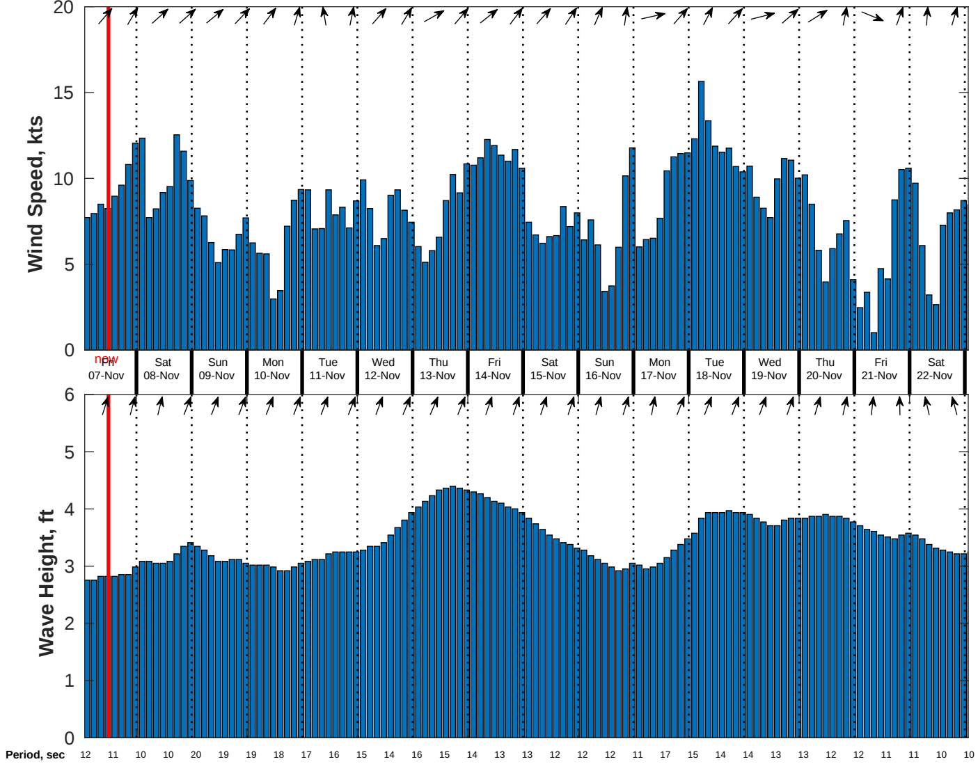
Wind & Wave Forecast for CSA (ONHYM) PPL EBS - Cote d'Ivoire from 06-Nov-2025 01:00:00 to 22-Nov-2025 01:00:00
