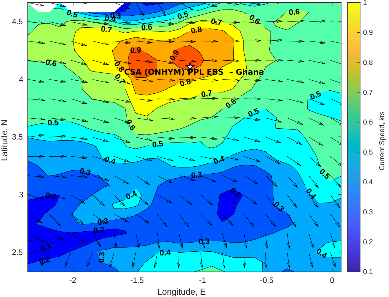
Surface Currents for CSA (ONHYM) PPL EBS - Ghana at 05-Nov-2025 00:00:00
