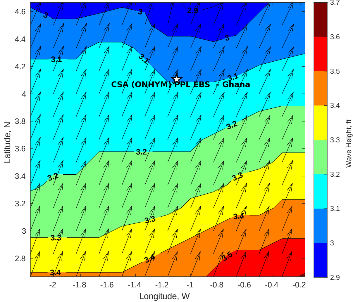
Wave Height (ft) for CSA (ONHYM) PPL EBS - Ghana at 06-Nov-2025 09:00:00
