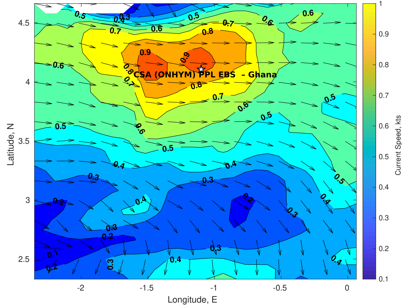
Surface Currents for CSA (ONHYM) PPL EBS - Ghana at 05-Nov-2025 00:00:00
