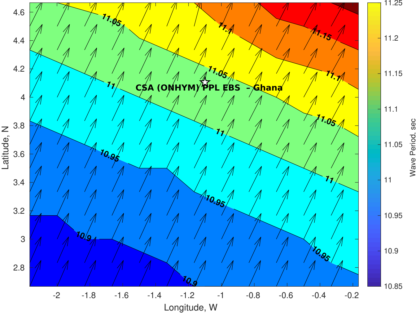
Wave Period (sec) for CSA (ONHYM) PPL EBS - Ghana at 06-Nov-2025 09:00:00
