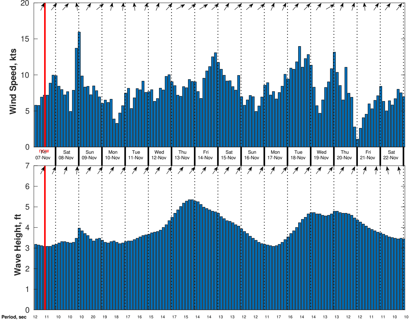
Wind & Wave Forecast for CSA (ONHYM) PPL EBS - Ghana from 06-Nov-2025 02:00:00 to 22-Nov-2025 02:00:00
