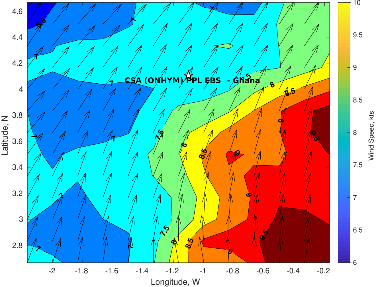
Winds (kts) for CSA (ONHYM) PPL EBS - Ghana at 06-Nov-2025 09:00:00
