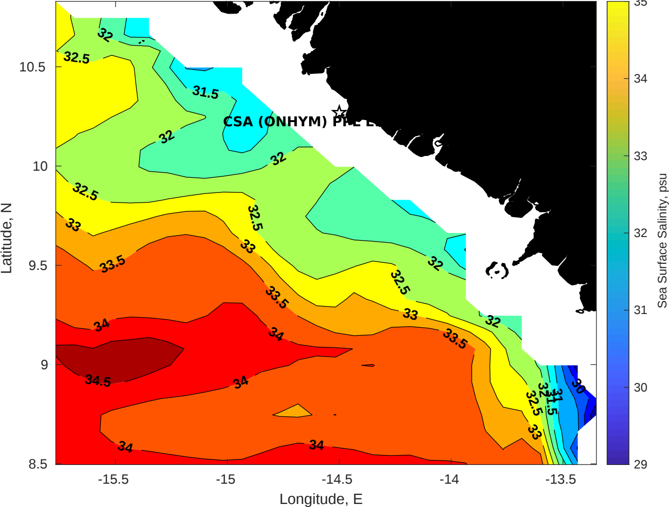
Surface Salinity for CSA (ONHYM) PPL EBS - Guinea at 05-Nov-2025 00:00:00
